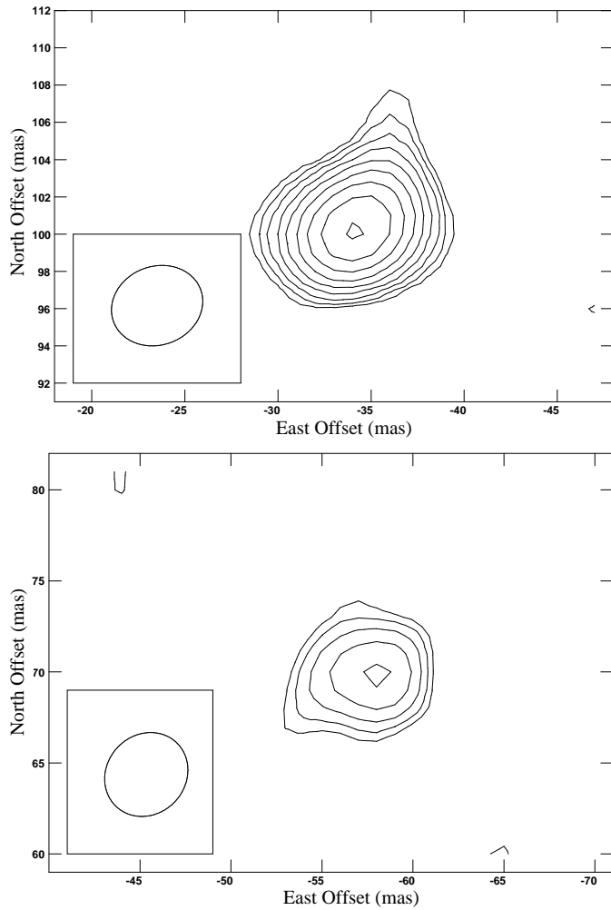
Fig. 6. Phased-referenced images for two background sources belonging to maser L 1206, J2223+6249 (top) and J2225+6411 (bottom) in the fifth epoch. Position offset (0,0) corresponds to the position listed in Table 2. Contour levels start at a 3\sigma level, 3.5 and 0.5 mJy beam ^{-1} respectively, and increase by factors of \sqrt{2} .
