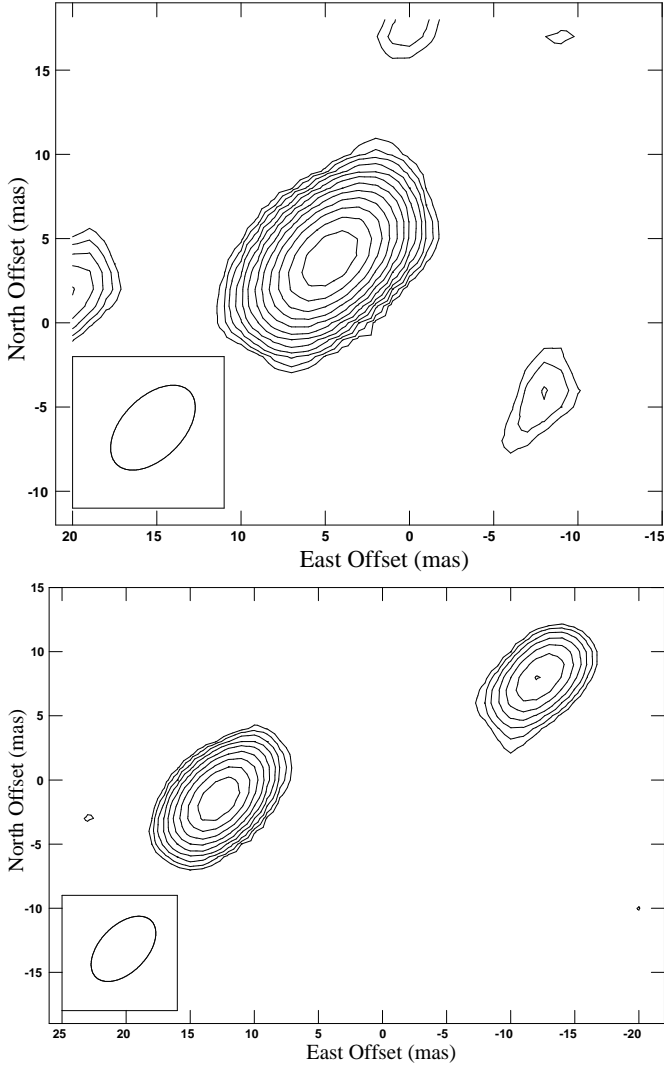
Fig. 14. Phased-referenced images for two background sources belonging to maser NGC 281-W, J0047+5657 (top) and J0052+5703 (bottom) in epoch five. Position offset (0,0) corresponds to the position listed in Table 2. Contour levels start at a 3\sigma level, 2.8 and 0.6 mJy beam -1 respectively, and increase by factors of \sqrt{2} . The bottom image shows also the additional component \sim 25 mas westward of J0052+5703.
