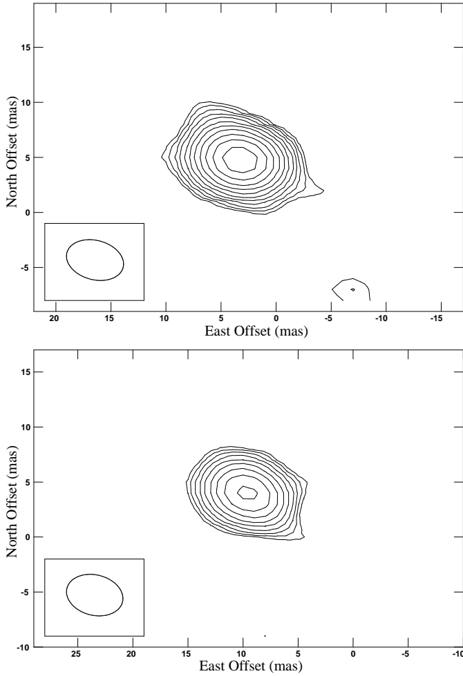
Fig. 2. Phased-referenced images for two background sources belonging to maser ON 1, J2003+3034 (top) and J2009+3049 (bottom) in the third epoch. Position offset (0,0) corresponds to the position listed in Table 2. The contour levels start at a 3\sigma level, 6.1 and 0.6 mJy beam ^{-1} respectively, and increase by factors of \sqrt{2} .
