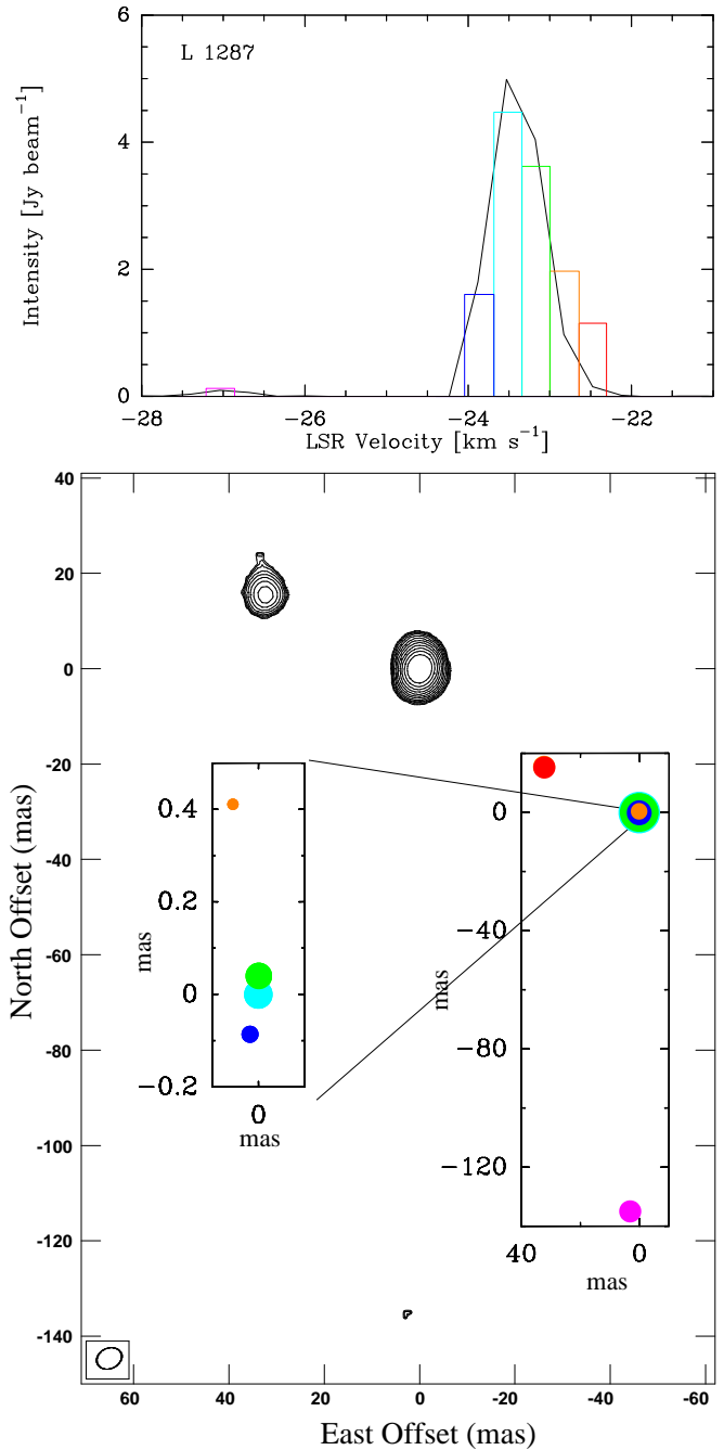
Fig. 9. Velocity integrated map and the spectrum of L 1287. Position offset (0,0) corresponds to the position listed in Table 2. Maser spots are indicated with color codes for different radial velocities. The areas of the colored circles and the colored histogram entries in the spectrum are scaled to the peak flux of that spot. Note that the black line in the spectrum is the intensity of the maser within a selected surface, which is not necessary the same as the intensity of the maser spot retrieved from a Gaussian fit. Contour levels start at 0.05 Jy beam ^{-1} km s ^{-1} and increase by factors of \sqrt{2} .
