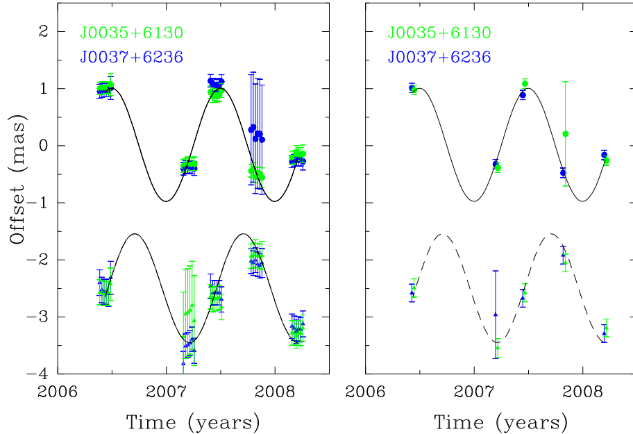
Fig. 11. Results of the parallax fit for L1278 based on six maser spots. The left graph shows a combined fit on all data, while the right graphs is a fit on the averaged data sets. The filled dots mark the data points in right ascension, while the filled triangles mark the declination. The solid line is the resultant fit in right ascension, the dashed line in declination. Different colors indicate a different background source.
