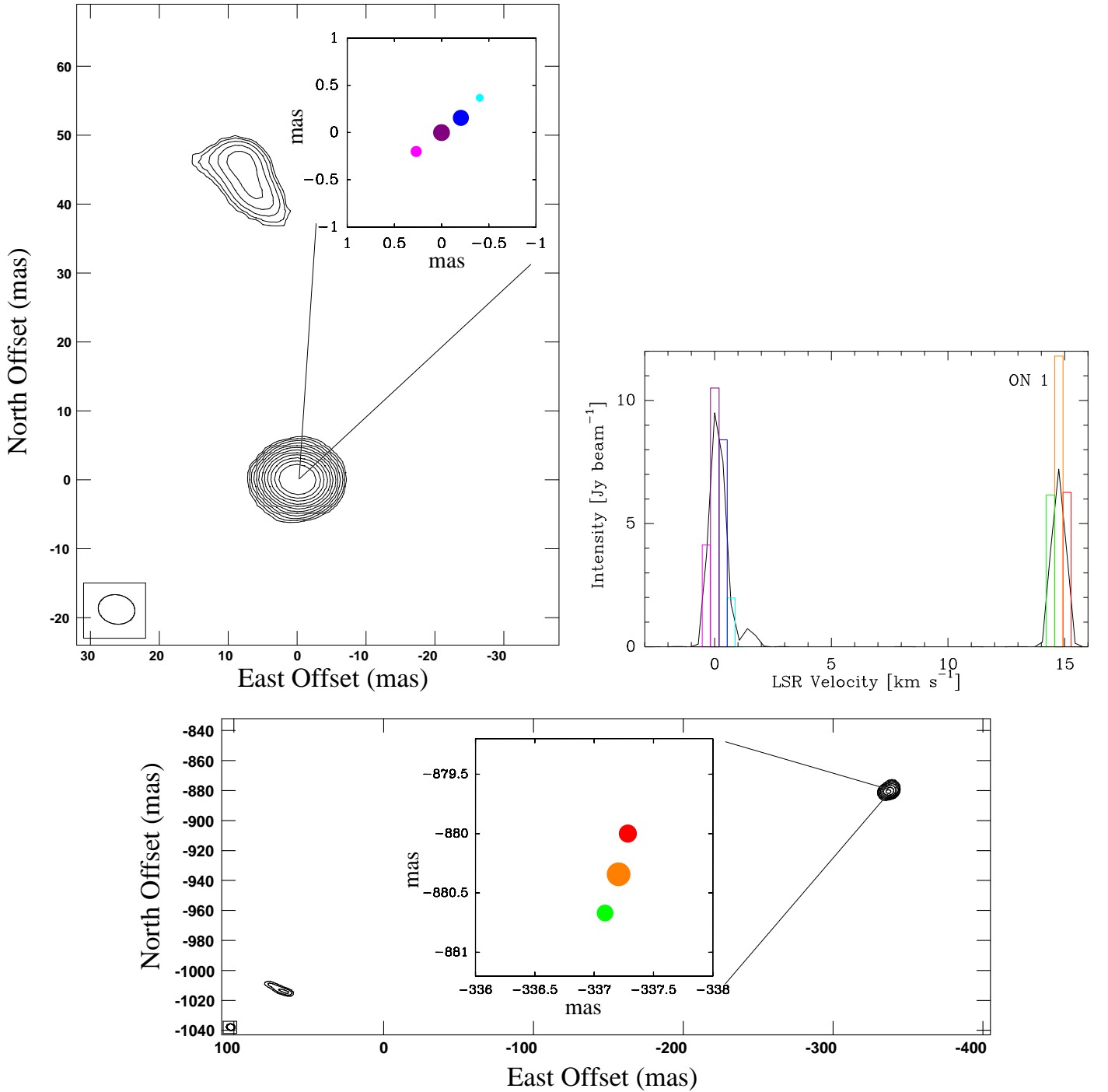
Fig. 1. Velocity integrated maser emission of the northern (up, left) and southern (bottom) maser groups in ON 1 together with the spectrum (up, right). Position offset (0,0) corresponds to the position listed in Table 2. Maser spots are indicated with color codes for different radial velocities. The areas of the colored circles and the colored histogram entries in the spectrum are scaled to the peak flux of that spot. Note that the black line in the spectrum is the intensity of the maser within a selected surface, which is not necessary the same as the intensity of the maser spot retrieved from a Gaussian fit. For the northern group, the contour levels start at 0.1 \text{ Jy beam}^{-1} \text{ km s}^{-1} , in the southern group, 1.0 \text{ Jy beam}^{-1} \text{ km s}^{-1} , and increase by factors of \sqrt{2} .
