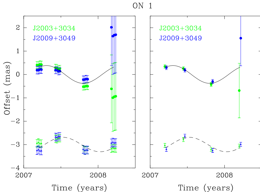
Fig. 3. Results of the parallax fit based on four maser spots. The left graph shows a combined fit on all data, the right graph is a fit on the averaged data sets. The filled colored dots mark the data points in right ascension, while the filled colored triangles mark the declination. The solid line is the resultant fit in right ascension, the dashed line in declination. Different colors indicate a different background source.
