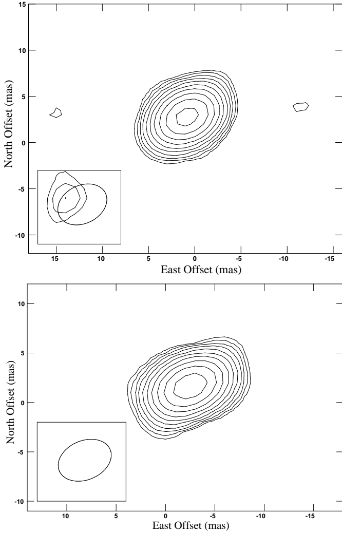
Fig. 10. Phased-referenced images for two background sources belonging to maser L 1287, J0035+6130 (top) and J0037+6236 (bottom) in epoch three. Position offset (0,0) corresponds to the position listed in Table 2. Contour levels start at a 3\sigma level, 3.6 and 2.4 mJy beam ^{-1} respectively, and increase by factors of \sqrt{2} .
