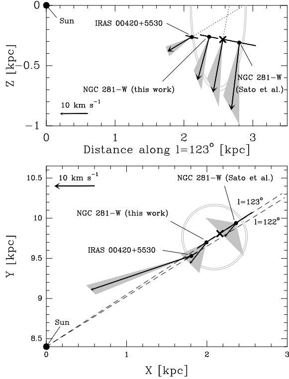
Fig. 21. The lower panel shows a face-on view of the Galactic plane. The Galactic longitudes of NGC 281-W ( l \approx 123^\circ ) and IRAS 00425530 ( l \approx 122^\circ ) are indicated by dashed lines. The top panel shows a cross-section of the Galactic plane along the Galactic longitude of NGC 281-W ( 123^\circ ). The vertical coordinate of this plot is the direction perpendicular to the Galactic plane. We plot NGC 281-W and IRAS 00420+5530 as black dots together with the respective distance error. Black arrows show the peculiar motion of the source, after removing the Galactic rotation ( R_0 = 8.4 kpc, \Theta_0 = 254 km s ^{-1} ). The errors in peculiar motion are indicated by the grey cones. The light-grey circles mark the super bubble with the center of the bubble at a distance of 2.5 kpc and a radius of 0.4 kpc, adopted after Sato et al. (2008). The cross marks the averaged distance of 2.58 kpc. The dotted lines show the backward prolongation of the proper motion of NGC 281-W and IRAS 00420+5530.
