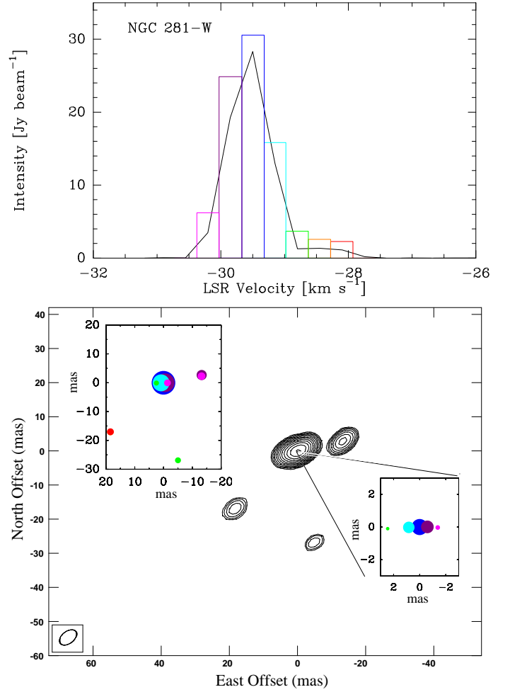
Fig. 13. Velocity integrated map and the spectrum of NGC 281-W. Position offset (0,0) corresponds to the position listed in Table 2. Maser spots are indicated with color codes for different radial velocities. The areas of the colored circles and the colored histogram entries in the spectrum are scaled to the peak flux of that spot. Note that the black line in the spectrum is the intensity of the maser within a selected surface, which is not necessary the same as the intensity of the maser spot retrieved from a Gaussian fit. Contour levels start at 0.5 Jy beam ^{-1} km s ^{-1} and increase by factors of \sqrt{2} .
