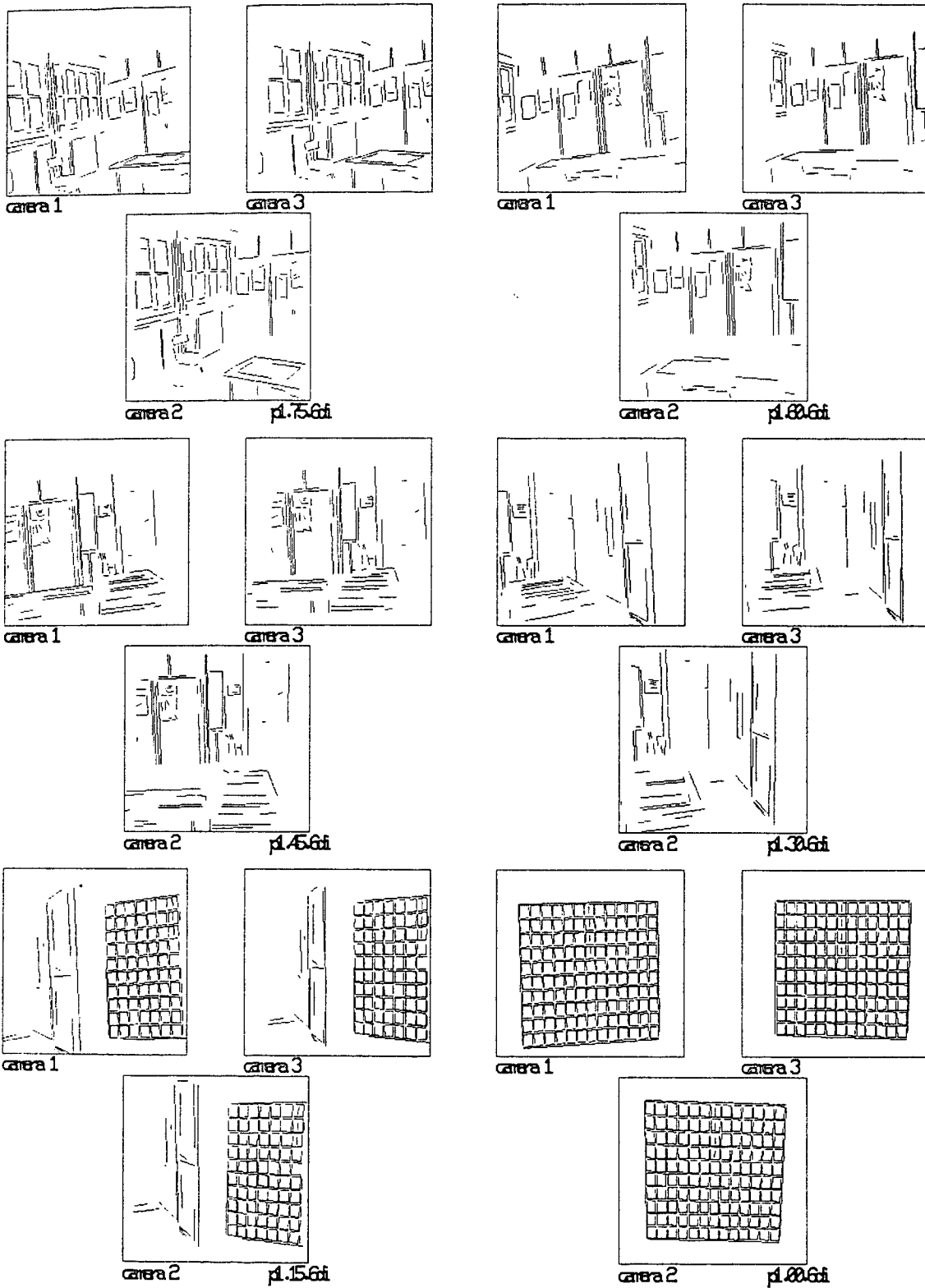
Figure 20: Matched segments
