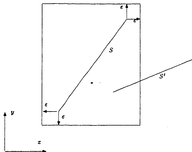
Figure 16: S' is \varepsilon -compatible with S iff it intersects the box
