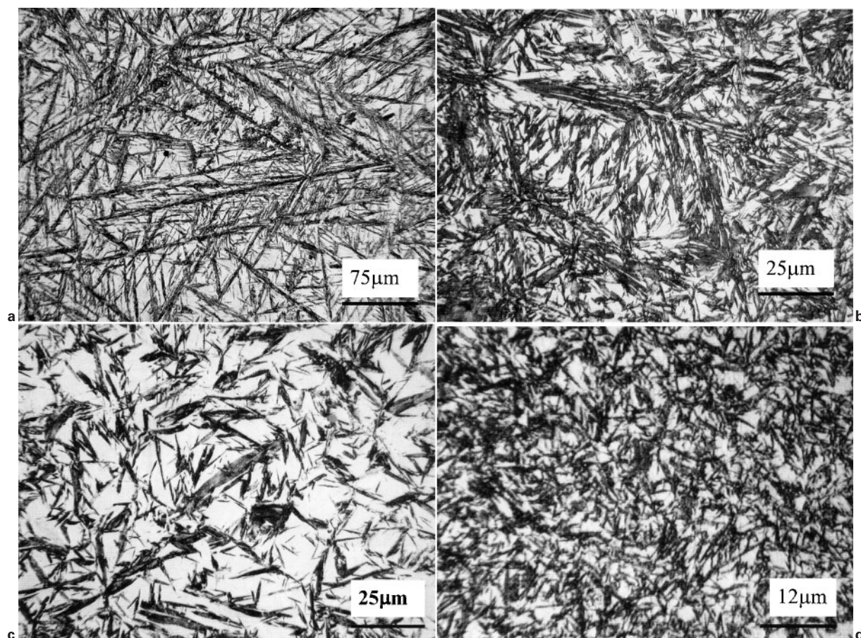
1 Optical micrographs of specimens quenched from a 1200, b 1100, c 1000 and d 950°C: note that micrographs are presented at different magnifications for clarity
