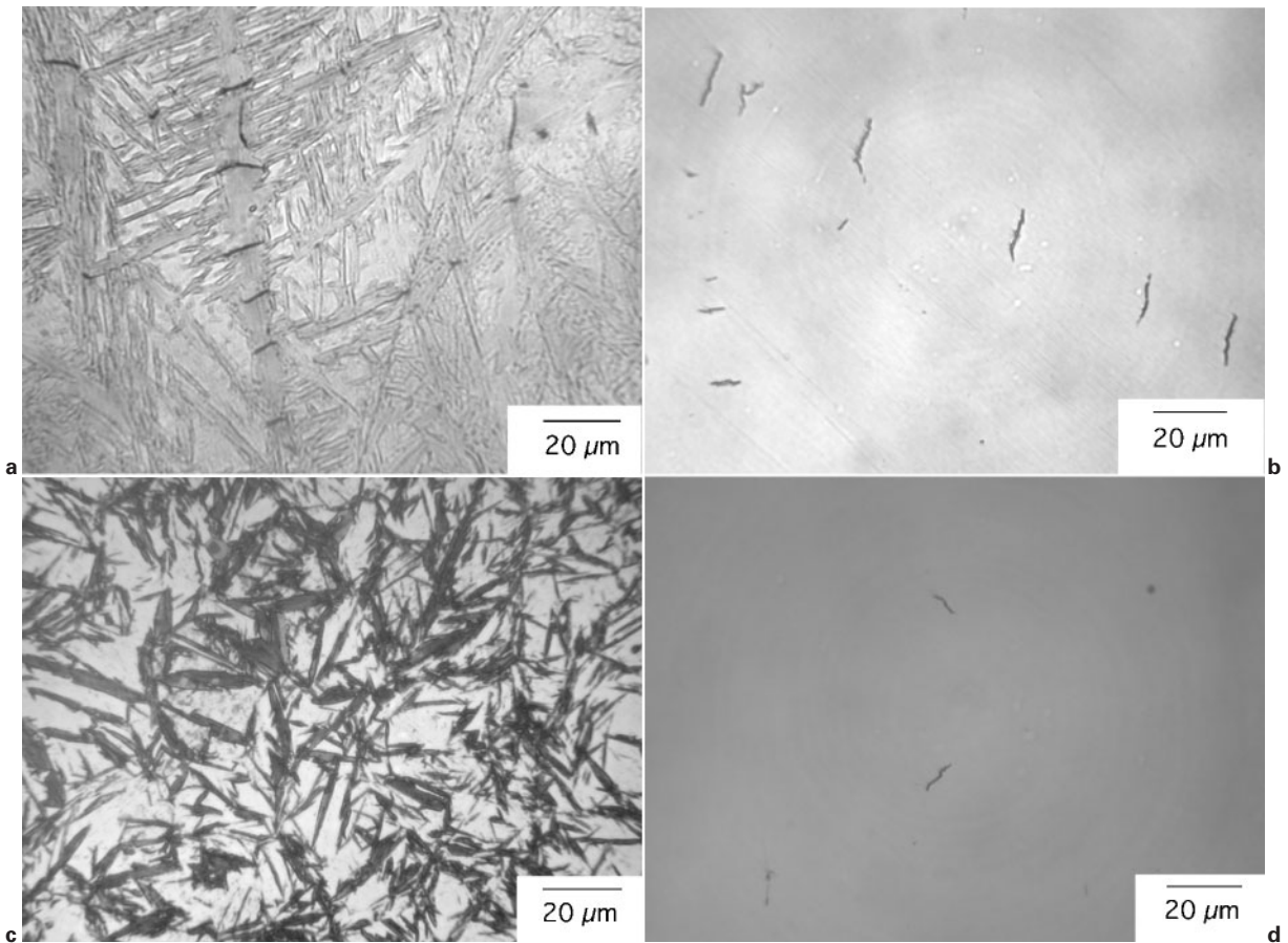
2 Microcracking in specimen austenitised at 1200°C: a etched specimen and b periodically cracked plate in unetched specimen; corresponding images for T_{\gamma}=1000^{\circ}\text{C} of c etched specimen where cracks are difficult to observe and d occasional cracks visible in unetched specimen
