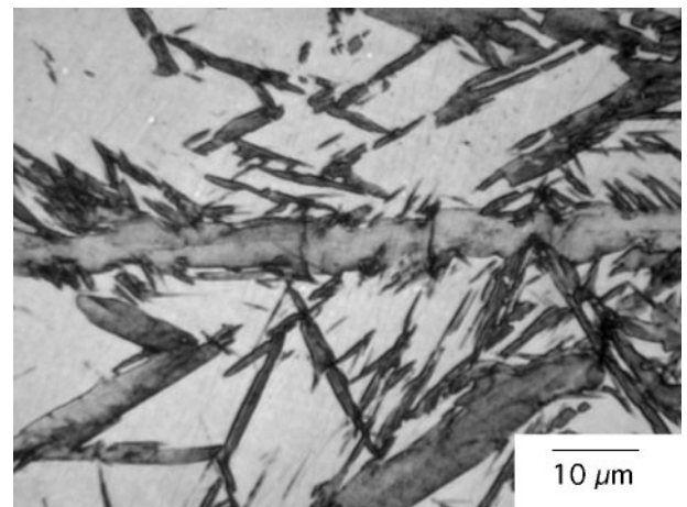
3 Microcracking in specimen austenitised at 1200°C and soaked at 950°C before quenching
