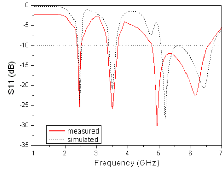
Figure 3. Simulated and measured S_{11} for the proposed antenna.
