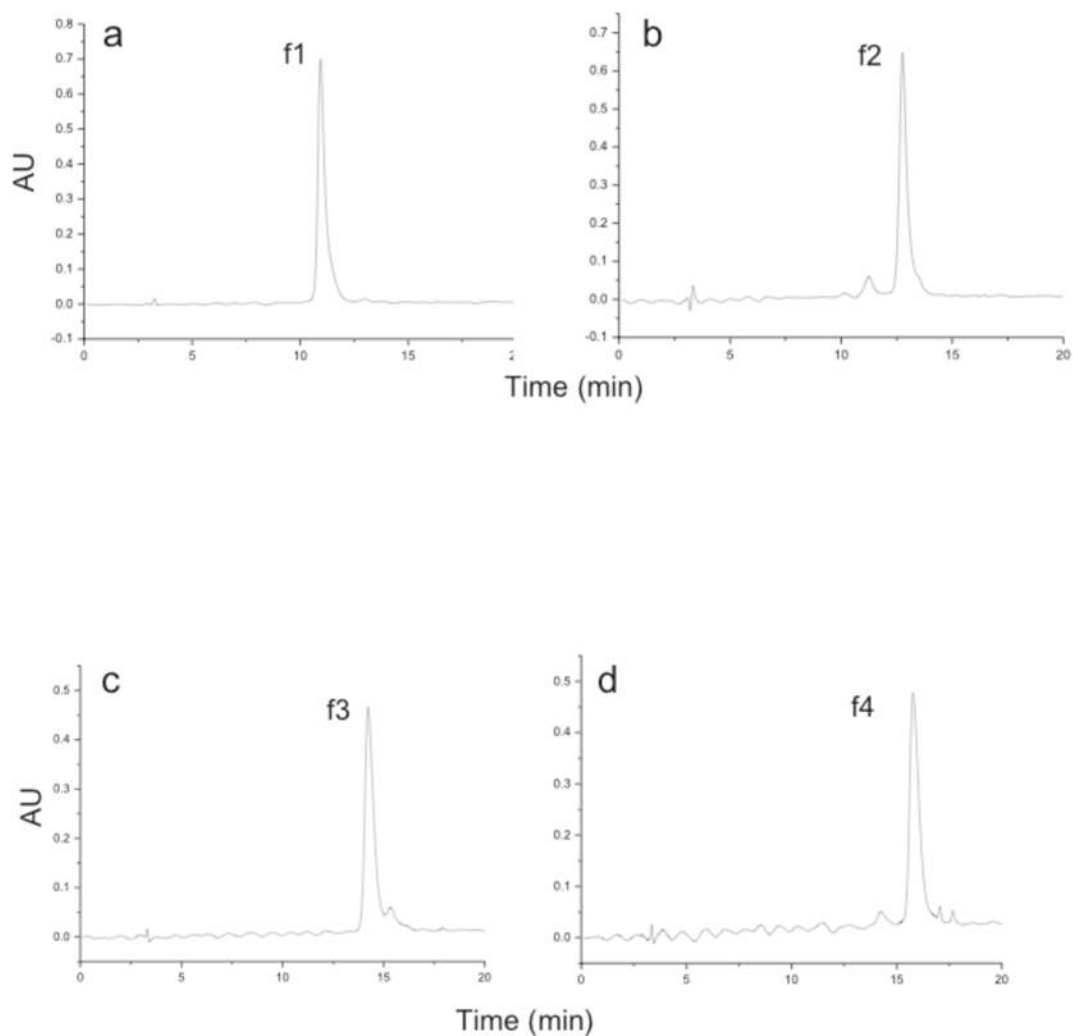
Figure 5. PDA RP-HPLC analysis of isolated (a) f1, (b) f2, (c) f3, and (d) f4 products (see designations in Figure 4). PDA RP-HPLC was performed using a C_{18} RP column, an elution gradient of 10–30% B in 20 min, and a flow rate of 1.0 mL/min. Eluants were 0.1% TFA in water (A) and 0.1% TFA in acetonitrile (B). Other conditions are given in Material and Methods.
