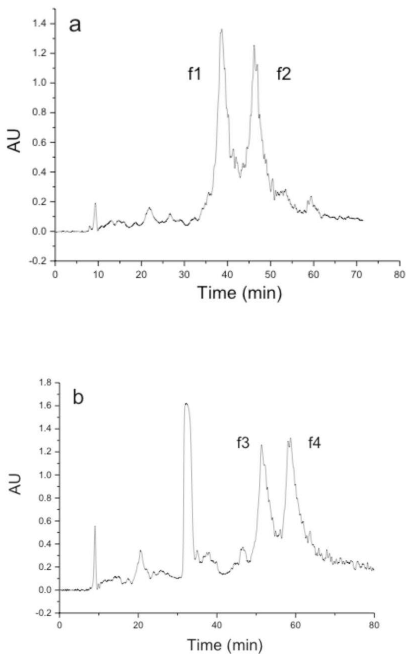
Figure 4. Semi-preparative RP-HPLC analysis of (a) phosphinate triple-helical peptide and (b) phosphinate triple-helical peptide-amphiphile. Semi-preparative RP-HPLC was performed using a C 18 RP column, an elution gradient of 10–30% B in 80 min, and a flow rate of 10.0 mL/min. Eluants were 0.1% TFA in water (A) and 0.1% TFA in acetonitrile (B). Detection was at \lambda = 220 nm. Other conditions are given in Material and Methods.
