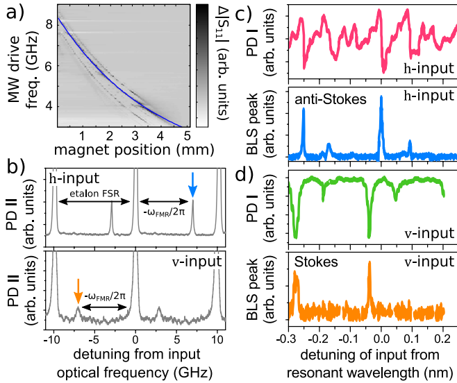
Figure 3. (a) FMR of YIG sphere measured through microwave reflection coefficient |S_{11}| of the antenna as a function of permanent magnet position. The blue dashed line shows the expected dependence of the uniform Kittel mode from the known dependence of magnetic field on distance from a cuboid magnet [26] and the gyromagnetic ratio \gamma = 28 \text{ GHz T}^{-1} . The magnetic field range is H_{dc} \approx 100\text{-}320 \text{ mT} . The Q -factor of the magnetic mode is Q_{\text{FMR}} \approx 400 (as this is due to Gilbert damping, the rate \kappa_{\text{FMR}} \approx 10\text{-}20 \text{ MHz} depends linearly on FMR frequency [27]). (b) Measured spectra of emitted signal (PD II) for h (upper) an v input polarization for \omega_{\text{FMR}}/2\pi \approx 7 \text{ GHz} . Orange and blue arrows label Stokes and anti-Stokes peaks, respectively. We can exclude the suppressed side-band down to the signal-to-noise ratio, maximum \approx 20 (slightly different for the two input polarizations due to different experimental conditions). (c,d) Lower panels: maximum of BLS intensity as a function of input laser wavelength, for h and v input, respectively. Upper panels: Reflected optical intensity (PD I), shown for comparison. The x -axes is detuning from the resonant wavelength of the h polarized mode. For v input measurements, this is set by the measured h - v splitting \lambda_{h-v}^{\text{eff}} . For the optical modes Q_v \approx 2 \times 10^5 and Q_h \approx 1 \times 10^5 (dissipation rates \kappa_v \approx 1 \text{ GHz} , \kappa_h \approx 2 \text{ GHz} ).
