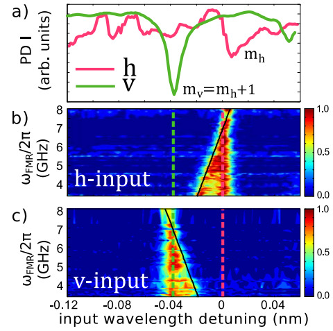
Figure 4. BLS scattering amplitudes for different input linear polarizations ( h : pink, v : green). (a) Reflected intensity (PD I) for comparison. Azimuthal mode indices are labeled for clarity. The two curves are plotted on separate scales. (b) Color-plot of BLS intensity for h -input polarization as a function of input laser wavelength and FMR frequency. Each scan for fixed FMR frequency has been normalized to the peak amplitude for that scan. (c) As in (b), but for v -input polarization. Dashed lines in (b) and (c) indicate the resonant wavelengths for the two polarizations. The x -axis in all panels is in detuning from the resonant wavelength of the h polarized mode. For v input measurements, this is set by the measured h - v splitting.
