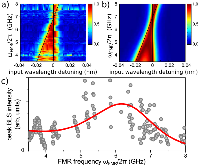
Figure 5. Comparison between (a) experiment and (b) theory of BLS intensity as a function of input wavelength detuning and FMR frequency for h input polarization. The black lines are the wavelengths corresponding to \omega_h and \omega_v - \omega_{\text{FMR}} . Both experimental data and model are normalized to the peak value at each FMR frequency to allow better comparison of the mode structure. (c) Peak BLS efficiency as a function of FMR frequency. The red line is the expected trend given by the maximum of Eq. (2) for fixed \omega_{\text{FMR}} .
