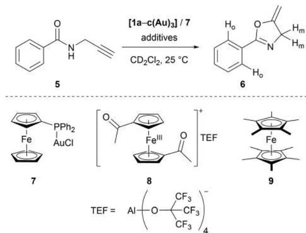
Scheme 2 Gold(I)-catalysed ring-closing isomerisation of N -(2-propyn-1-yl)benzamide 5 to oxazoline 6 (top, labelled protons used for following the reaction), including alternative mononuclear (pre-)catalyst 7 , oxidant 8 , and reductant 9 .
