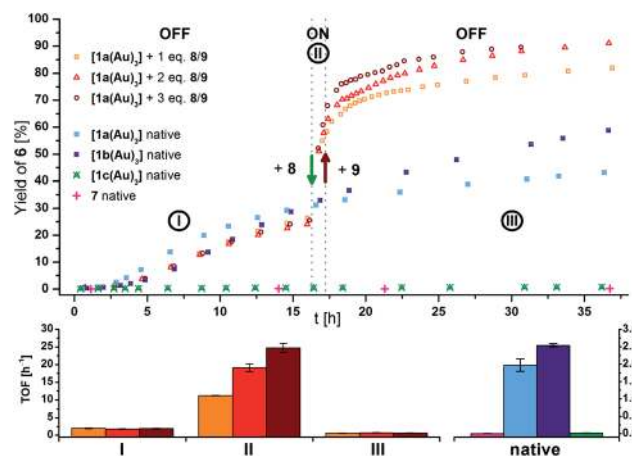
Fig. 4 (Top) Yield-over-time graphs for native (crossed symbols) and redox-switchable (hollow symbols) gold(I)-catalysed cyclisation of 5 to 6 (3 mol% Au as [\mathbf{1a}(\text{Au})_3] and 7 , [\mathbf{5}]_0 = 60 \text{ mmol L}^{-1} , \text{CD}_2\text{Cl}_2 , 25^\circ\text{C} ). Arrows indicate the addition of additives. I: initial OFF phase with little catalytic activity; II: ON phase after addition of 1.0–3.0 eq. oxidant 8 ; III: 2 nd OFF phase of little catalytic activity after addition of 1.1–3.3 eq. reductant 9 . (Bottom) Comparison of turnover frequencies (TOF), determined from linear fits of fixed time frames (s. Fig. S39–S45 † ) for the switched reaction phases shown above (left) and for the native complexes (right).
