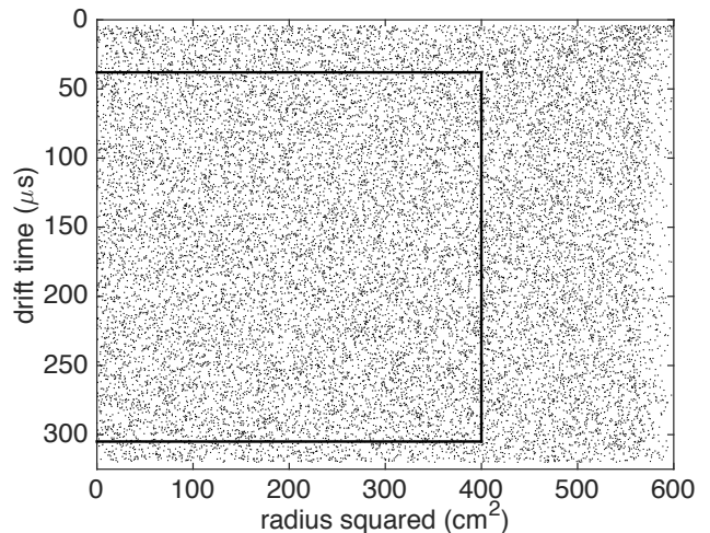
FIG. 3: The location of events in drift time vs. detector radius squared for the August 2013 \text{CH}_3\text{T} injection. The drift time is a proxy for the z coordinate of the event. The solid black line represents the fiducial volume used in Ref. [3].
