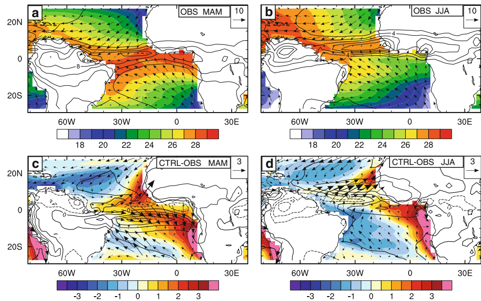
Fig. 1 Climatological mean surface fields in MAM (left panels) and JJA (right panels). The top row (a, b) shows ICOADS SST (shading; °C), ICOADS surface winds (vectors; reference vector 10 m/s), and CMAP precipitation (contours; interval 1 mm/day). The bottom row (c, d) shows biases in CTRL relative to the observations (a, b). The contour interval for precipitation biases is 2 mm/day. Dashed contour lines indicate negative values
