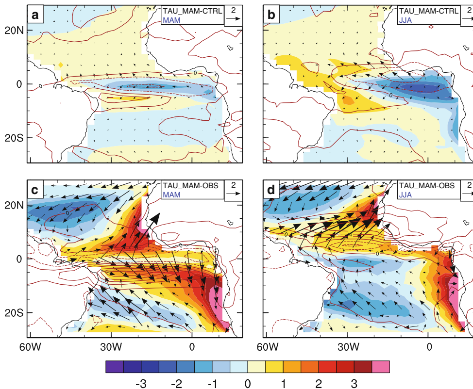
Fig. 5 SST (shading; K), surface wind (vectors; reference vector 2 m/s), and precipitation (contours; contour interval 1 mm/day) in MAM (left panels) and JJA (right panels) for experiment TAU_MAM,
