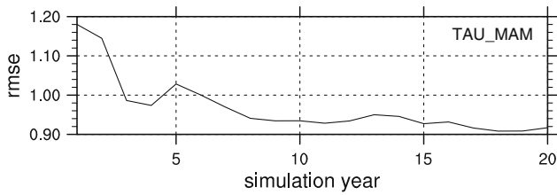
Fig. 3 Cumulative average of the RMSE of equatorial Atlantic SSTs (2°S–2°N) in experiment TAU_MAM relative to CTRL, plotted as a function of accumulation year. Thus, the value for year 5 corresponds to the average over years 1–5, the value for year 10 corresponds to the average over years 1–10, etc
