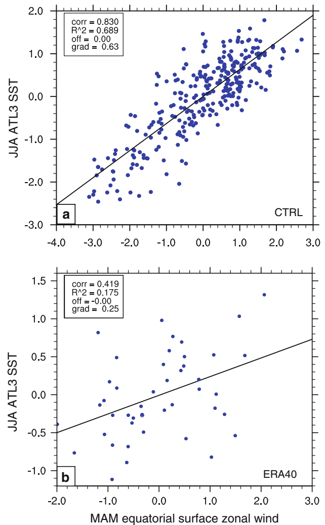
Fig. 8 Scatter plots of MAM equatorial surface winds averaged over the area (35°W–25°W, 3°S–3°N) and JJA ATL3 SST for a CTRL, and b ERA-40 reanalysis. Each dot corresponds to an individual year
