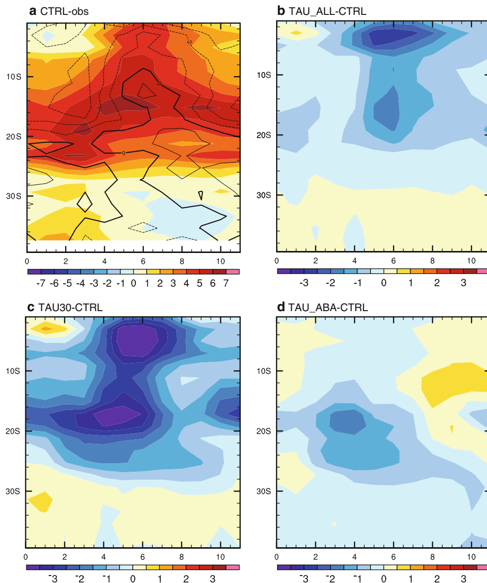
Fig. 12 Latitude-time sections of SST differences ( shading ; K), averaged between 8°E and the African coast. The individual panels show the differences of a CTRL and ICOADS, b TAU_ALL and
