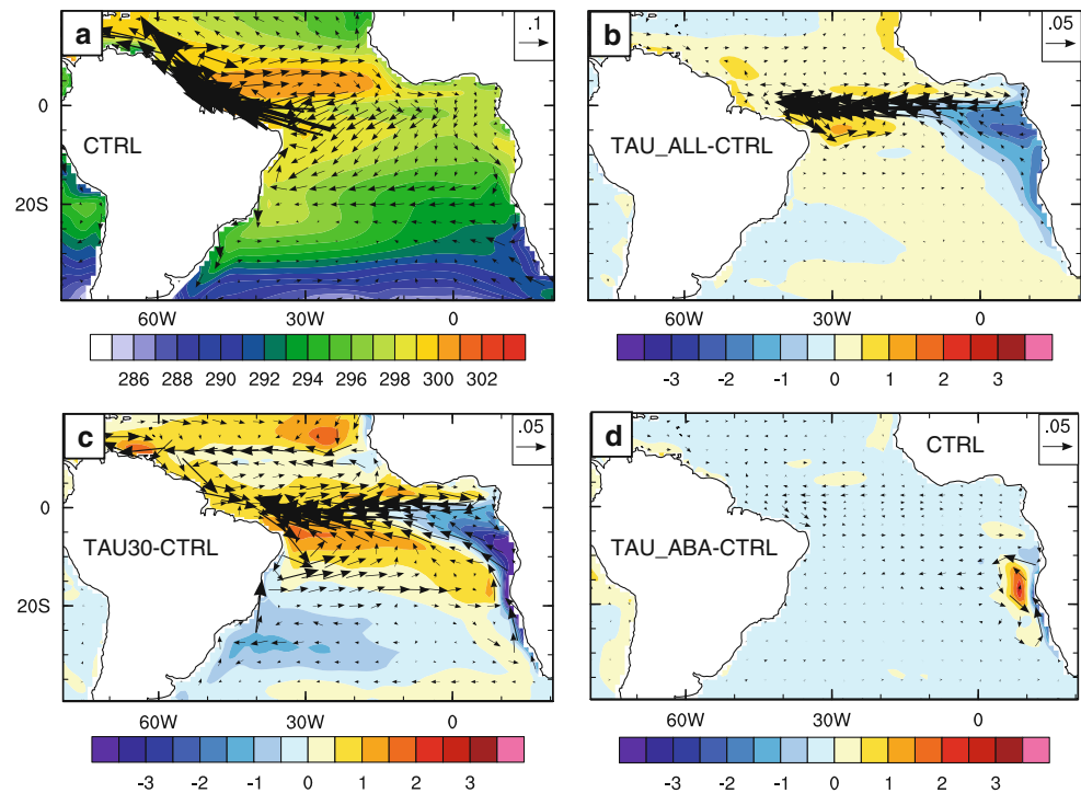
Fig. 13 Horizontal maps of annual mean potential ocean temperature ( shading ; K), and ocean currents ( vectors ; reference vector in m/s) averaged between 0 and 50 m. The individual panels show a CTRL, and the differences relative to CTRL for b TAU_ALL, c TAU30, and d TAU_ABA
