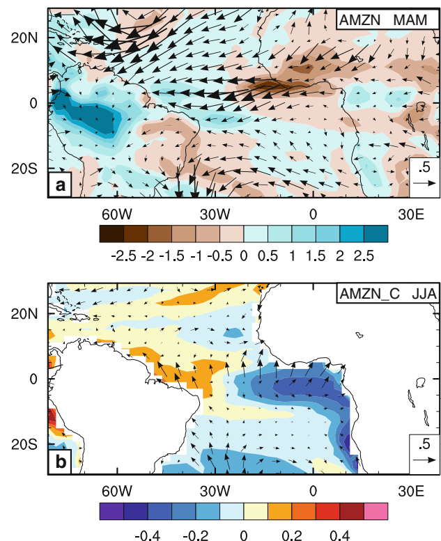
Fig. 9 Difference, relative to CTRL_A/CTRL, of surface winds (vectors; reference vector 0.5 m/s) and a precipitation (shading; mm/day) and b SST (shading; K) for experiments AMZN and AMZN_C, which set surface albedo to 0 in the Amazon region. a Shows MAM for AMZN, while b shows JJA for AMZN_C, the coupled counterpart to AMZN
