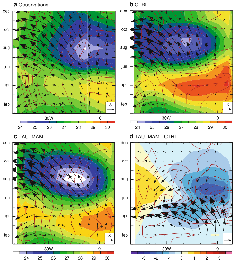
Fig. 4 Longitude-time sections along the equator (averaged from 2°S–2°N) of SST (shading; K), surface wind stress (vectors; N\ m^{-2} * 10 ), and depth of the 20°C isotherm (contours; contour interval 5 m). The individual panels show a observations (ICOADS SST and wind stress, WOA thermocline depth), b CTRL (300-year mean), c TAU_MAM (20-year mean), and d the difference between TAU_MAM and CTRL
