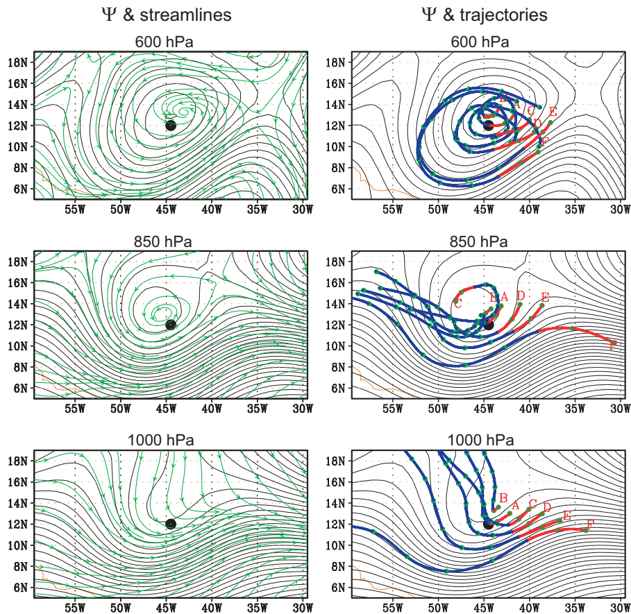
Fig. 18. Streamlines and trajectories of horizontal (rotational + divergent) flow at (a, b) 600 hPa, (c, d) 850 hPa, and (e, f) 1000 hPa as seen in ERA-40 data, for the average of six consecutive leading up to the best-track genesis time of Hurricane Debby (2000). As in Fig. 5, the streamlines (shown in panels a, c, e) are calculated and displayed in a frame of reference moving westward with the parent wave. Translation speeds estimated from the Hovmöller method at the three levels are -9.1 \pm 0.3 \text{ ms}^{-1} (600 hPa), -10.0 \pm 0.6 \text{ ms}^{-1} (850 hPa) and -10.1 \pm 0.6 \text{ ms}^{-1} (1000 hPa). Likewise the stream function of non-divergent flow (thin solid) and trajectories (shown in panels b, d, f) are calculated and is displayed in the co-moving frame. The contour interval for stream function is 0.5 \times 10^6 \text{ m}^2 \text{ s}^{-1} . The genesis location is indicated by the black dot in each panel. Note that owing to the translation of sequential frames used to construct the time average when C_p \neq 0 , the longitude labels on the x-axis pertain to the final analysis time only.
