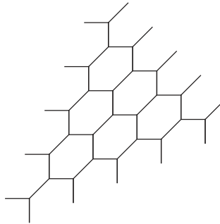
Figure 1. The tropical plane quintic curve that describes part of the discriminant \mathcal{A} of \partial\Delta .
