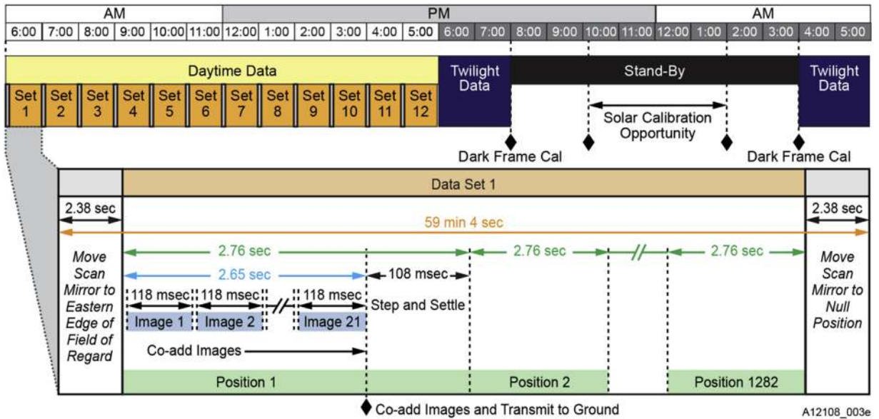
Fig. 7. Nominal daily operations for TEMPO instrument.
