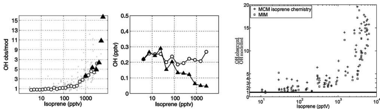
Fig. 10 (Left) The observed-to-modelled OH ratio as a function of isoprene with open circles showing data taken at <1 km altitude and SZA < 60^\circ during INTEX-A and filled triangles showing data from PROPHET-2000 (ground-based). (Middle) The median observed OH (circles) and modelled OH (triangles) during INTEX-A as a function of isoprene. (Right) Observed to modelled ratio of [OH] during the GABRIEL campaign over the Suriname rainforest as a function of isoprene concentration, for two different models. (Reproduced from ref. 182, Copyright (2008) American Geophysical Union, reproduced by permission of American Geophysical Union (further reproduction or electronic distribution is not permitted) and ref. 196, Copyright (2010), with permission from Copernicus Publications.)
