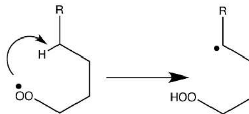
Figure 39. \text{RO}_2 isomerisation to QOOH. In this mechanism, well known in combustion chemistry, the terminal O atom of the \text{RO}_2 abstracts a labile H (through the formation of a ring-structured intermediate).
