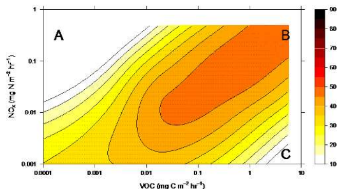
Figure 4. O 3 mixing ratios (ppb) as a function of VOC and NO x emissions as computed using the UKCA model of atmospheric chemistry (Archibald et al., 2011). Three main regions are identified. Top left corner (A): region of NO x saturation and O 3 titration. Bottom right corner (C): region of VOC saturation and O 3 destruction. Diagonal elements (A–C, B–C): efficient conversion of NO–NO 2 and hence O 3 production increasing with increasing VOC and NO x emissions (NB: log 10 scales for emissions).
