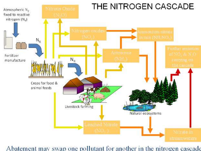
Figure 34. The nitrogen cascade adapted from Sutton et al. (2011) showing the interrelationships of nitrogen sources of importance for the production of ozone.
