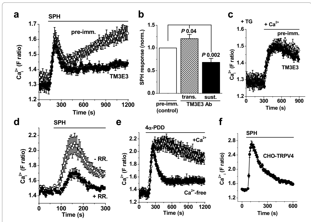
Figure 3 Inhibition of sustained sphingosine responses by anti-TRPM3 antibody in HIG-82 cells. Data were generated by intracellular Ca^{2+} measurement. (a) Cells were pre-treated with 1:4000 dilution of pre-immune serum (pre-imm.) or anti-TRPM3 antiserum before observing responses to 20 \mu M sphingosine (SPH). (b) Summary normalised data from 8 independent experiments showing inhibitory effect of TM3E3 on the sustained response to SPH. (c) Lack of effect of TM3E3 on Ca^{2+} entry in cells store-depleted by 1 \mu M thapsigargin (TG) for 30 min in Ca^{2+} -free extracellular solution followed by re-addition of 1.5 mM Ca^{2+} ; representative of N/n = 24/3 . (d-f) Investigation of the transient response to SPH. (d) Effect of 10 \mu M ruthenium red (+RR) on the SPH response in HIG-82 cells; representative of N/n = 12/3 . (e) Responses to 10 \mu M 4 \alpha -phorbol 12,13-didecanoate (4 \alpha -PDD) in HIG-82 cells in the presence (+ Ca^{2+} ) and absence of extracellular Ca^{2+} ; representative of N/n = 16/2 . (f) Representative of 3 independent experiments, responses to sphingosine (SPH, 20 \mu M ) in CHO cells stably expressing TRPV4.
