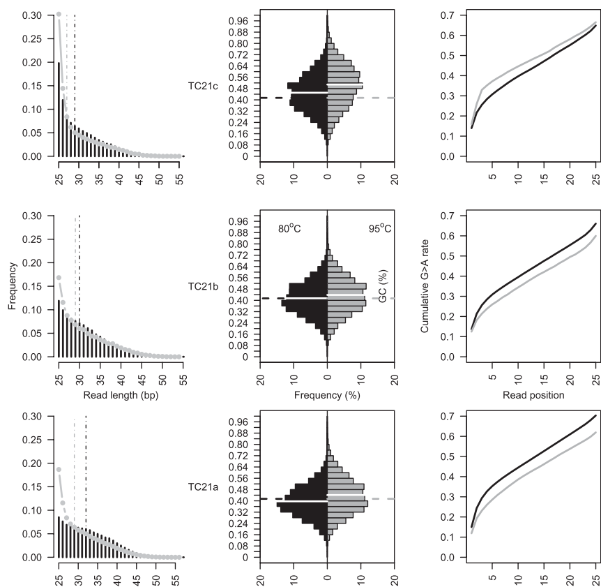
Figure 3. The distribution of Helicos reads is dependent on the initial denaturation temperature. Three different extracts ( top : TC21c; middle : TC21b; bottom : TC21a) have been sequenced on the same Helicos run (six channels) following identical procedures, except that either mild (80°C, black) or high (95°C, gray) temperatures were used for denaturation. ( Left ) Read length distribution. For extracts TC21c, TC21b, and TC21a, the median read size was 29, 30, and 32 bp when DNA denaturation was performed at 80°C (black dashed lines) in contrast to 27, 29, and 29 bp at 95°C (gray dashed lines). ( Middle ) Read GC contents. White full lines refer to average read GC contents; the expected genomic GC content (41.4%) is reported with dashed lines. ( Right ) Cumulative guanine to adenine misincorporation rates as a function of the distance from sequencing start.
