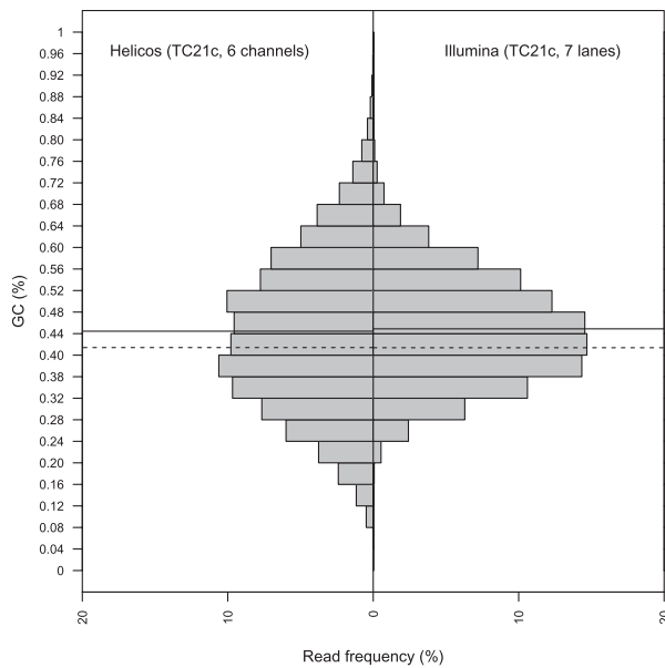
Figure 2. GC composition of Illumina and Helicos horse reads. For comparison, we considered only the reads generated from the same extract (TC21c) and denaturation temperatures of 80°C and 95°C. Similar distributions were recovered when considering the total number of Helicos reads generated for other extracts. ( Left ) Helicos; ( right ) Illumina. Full lines refer to the observed average read GC content. The expected average GC content of genomic fragments of 31 bp (Helicos read median) is estimated using 361,379 randomly sampled fragments of the horse reference genome (see Supplemental text) and is reported in dashed lines (41.41%). A similar estimate (41.38%) is provided for Illumina sequencing reads using 299,256 randomly sampled fragments of 67 bp, in agreement with the median of Illumina sequences.
