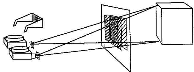
Fig 8. Left and right images can be projected on top of each other onto a silvered screen surface through separate polarizing lenses rotated 90° out of phase to each other. An audience wearing similarly aligned polarized glasses sees only the left image with the left eye and only the right image with the right eye.
