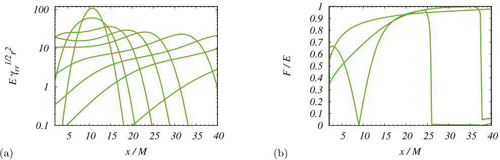
Fig. 2. (a) Evolution of the wave packet along the x and z axes for the initial condition (C-6) with F = 0 . The profiles are shown for t/M = 0, 5, 10, 15, 20, 30, 50, and 70 . (b) F/E along the x and z axes for t/M = 5, 20, and 50 . For both figures, the results for x and z axes agree approximately.
