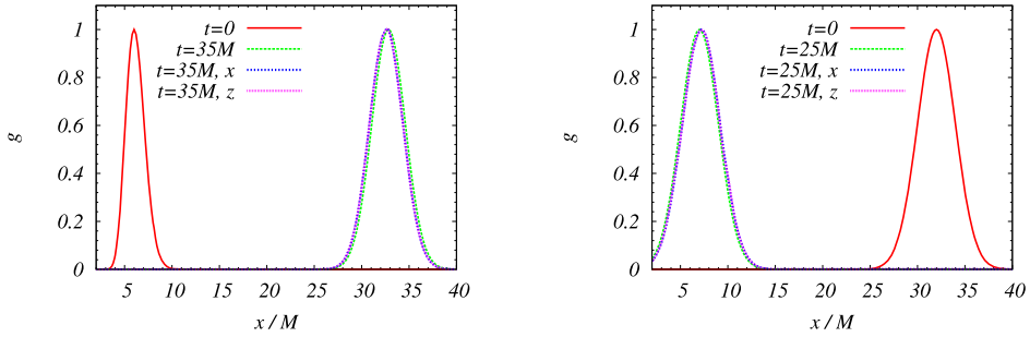
Fig. 1. Evolution of outgoing (left) and ingoing (right) solutions. For the outgoing solution, the profiles of E\gamma_{rr}^{1/2}(r - 2M)^2(1 + 2M/r)^{-3/2} at t = 0 and t = 35M along the x and z axes are plotted. For the ingoing solution, the profiles of E\gamma_{rr}^{1/2}r^{3/2}(r + 2M)^{1/2} at t = 0 and t = 25M along the x and z axes are plotted. The solid and dashed curves denote the numerical and exact solutions. The numerical solutions for x and z axes agree approximately.
