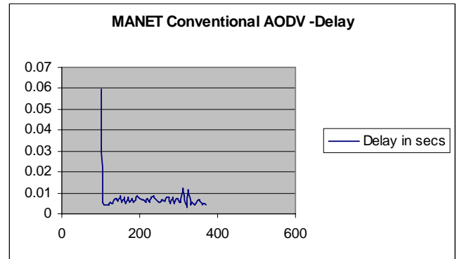
Fig. 1 AODV Delay
