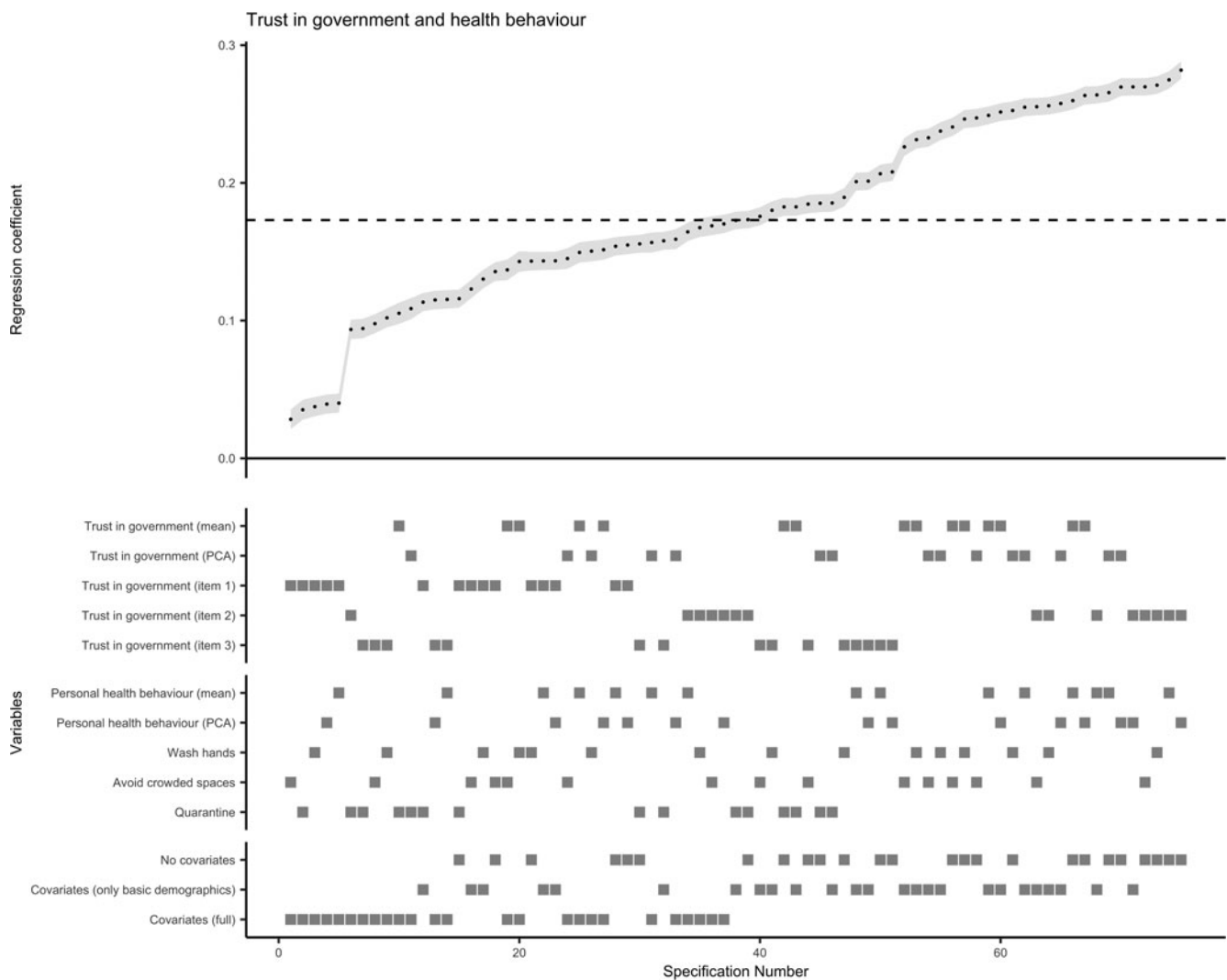
Fig. 3. Results of specification curve analysis for trust in government and adoption of personal health behaviour.
