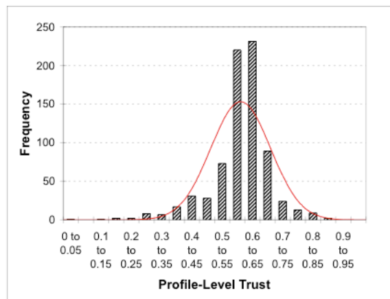
Figure 2: The distribution of profile-level trust values among the producer profiles.
