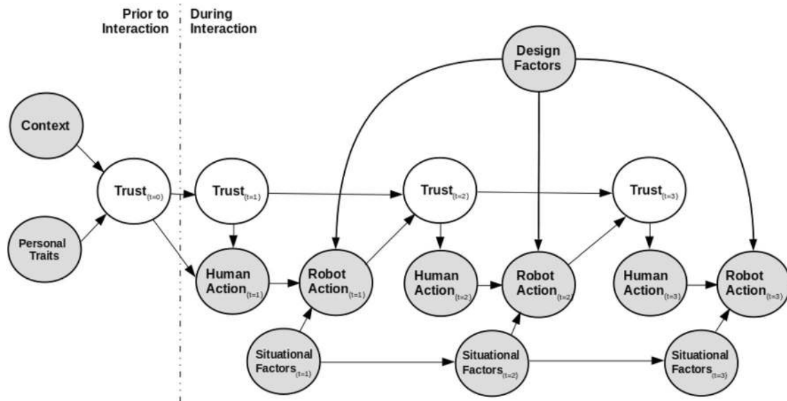
Fig. 5 A probabilistic graphical model (PGM) representation of Fig. 4 unrolled for three time steps. Latent variables (i.e., trust in the robot) are unshaded. Nodes can represent multidimensional random vectors. The graphical model encodes explicit assumptions about the generative process behind the interaction: conditional independence between any
