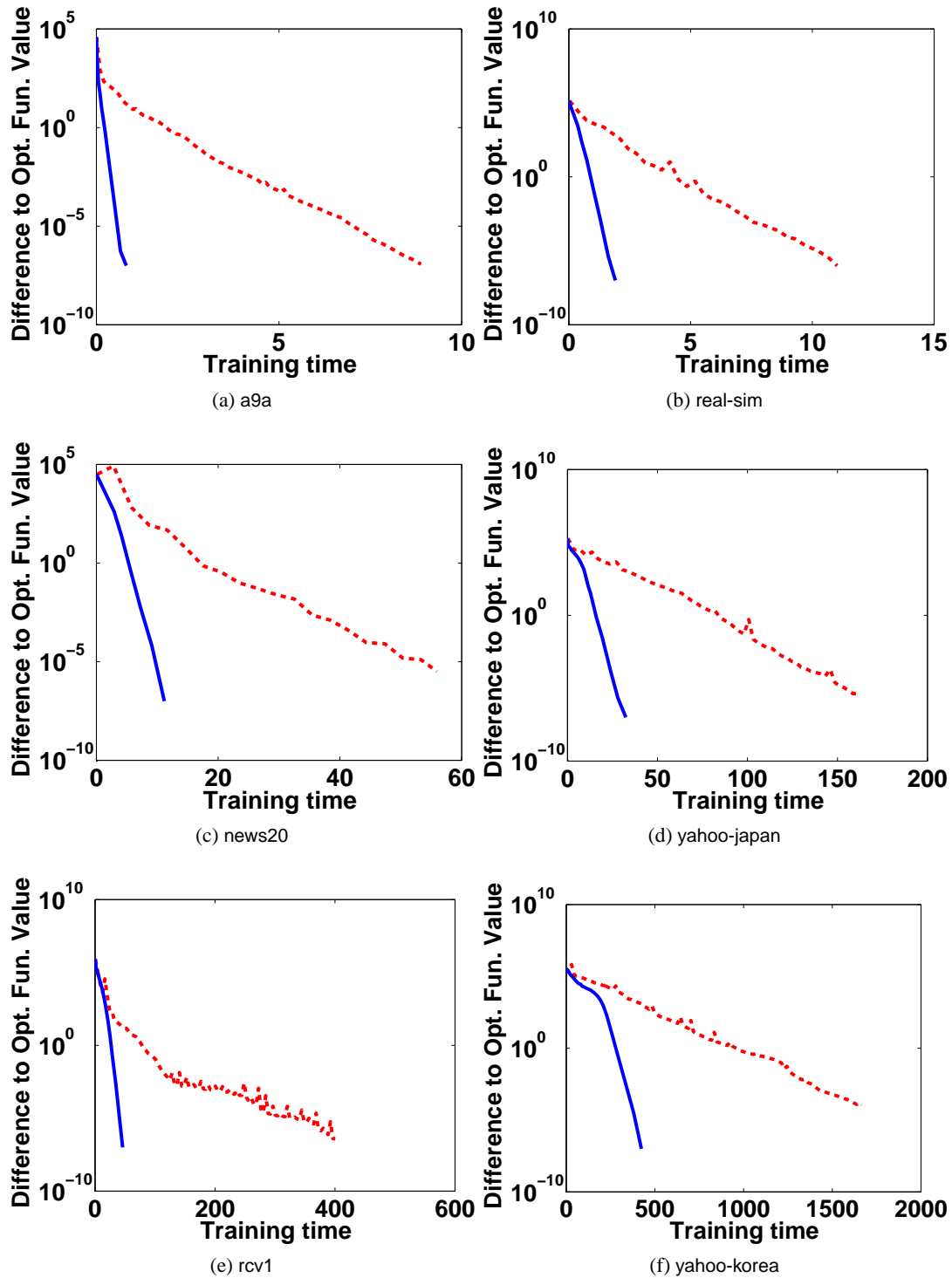
Figure 1: A comparison between TRON (blue solid line) and LBFSGS (red dotted line). The y-axis shows the difference to the optimal function value. The x-axis (training time) is in seconds. We use the training set from the first training/validation split of the CV procedure and set C = 4 .
