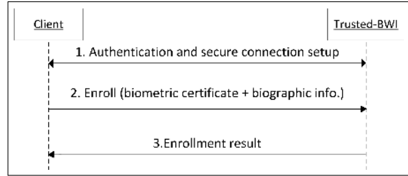
Figure 6. Sequence diagram of Trusted-BWI enrollment service.
