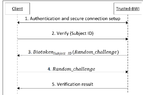
Figure 9. Sequence diagram of Trusted-BWI verification service relying on challenge and response authentication protocol using biotokens.
