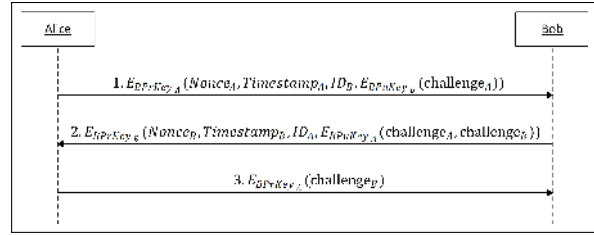
Figure 5. The remote authentication protocol using biometric public and private keys.
