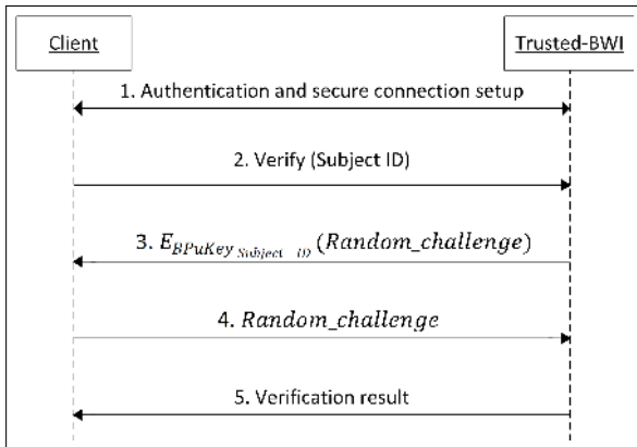
Figure 10. Sequence diagram of Trusted-BWI verification service relying on challenge-and-response authentication protocol using BKI's ABCS.
