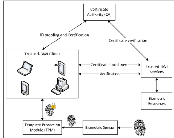
Figure 1. Overview of Trusted-BWI web services. An extended BKI uses a Template Protection Module (either software or hardware) which produces a Public Key/Private key and protects the private key, requiring biometric matching to use it. The CA does identity proofing with it, represented in the resulting certificate. The certificate can be enrolled in a Trusted-BWI server and used for later verification. The model allows trusting CAs for identity proofing; however, the Trusted BWI servers may also have their own CA. Privacy is maintained since traditional biometric data is not used outside the Template Protection Module. Stronger binding of digital certificates to identity, in a scalable manner, with privacy enhanced remote/client side matching, makes Trusted-BWI ideal for web-based applications needing trusted identities.
