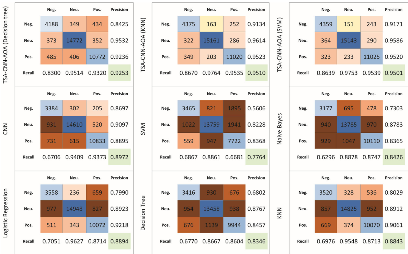
Fig. 10 Confusion matrices of all approaches
