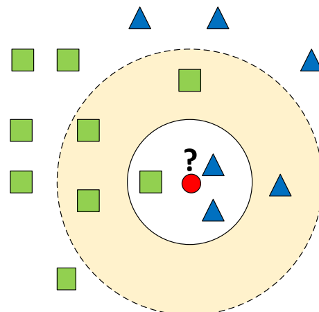
Fig. 3 An example of KNN classification algorithm
