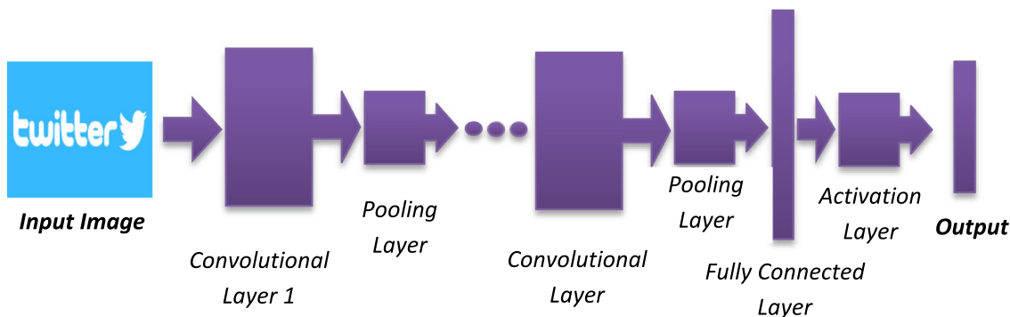
Fig. 1 CNN architecture
