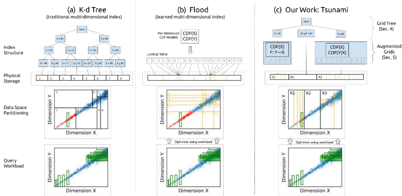
Figure 1: Indexes must identify the points that fall in the green query rectangle. To do so, they scan the points in red. (a) K-d tree guarantees equally-sized regions but is not optimized for the workload. (b) Flood is optimized using the workload but its structure is not expressive enough to handle query skew, and cells are unequally sized on correlated data. (c) Tsunami is optimized using the workload, is adaptive to query skew, and maintains equally-sized cells within each region.
