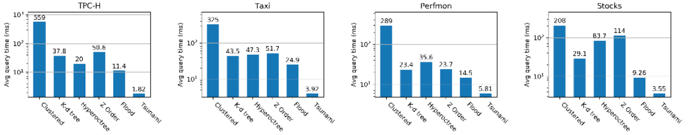
Figure 7: Tsunami achieves up to 6× faster queries than Flood and up to 11× faster queries than the fastest non-learned index.
