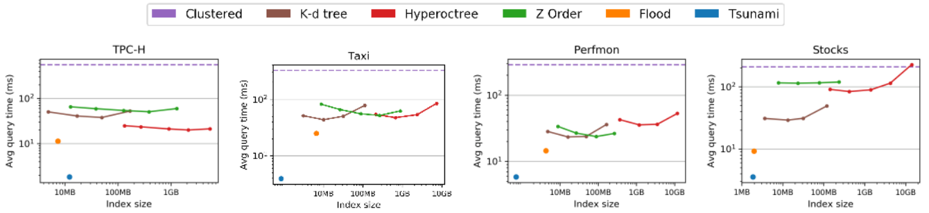
Figure 8: Tsunami uses up to 8× less memory than Flood and 7-170× less memory than the fastest tuned non-learned index.
