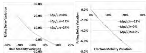
Figure 8: Inverter variation with mobility change.
