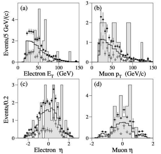
FIG. 31. E_T(p_T) and \eta distributions for electrons (muons) for leptonic t\bar{t} candidates (shaded histogram), t\bar{t} MC [HERWIG, m_t = 170 GeV/ c^2 ] (unshaded histogram), expected background (open triangles), and expected signal plus background (solid circles). The measured muon p_T for e\mu candidate 58796-7338(417) is 280.0 GeV/ c and is therefore off scale in plot (b). As given in Ref. [102], the event label corresponds to run number and event number (in an early event numbering scheme, this event became well known as “event 417” and thus retains this label parenthetically).
