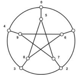
Fig. 3: Petersen graph
