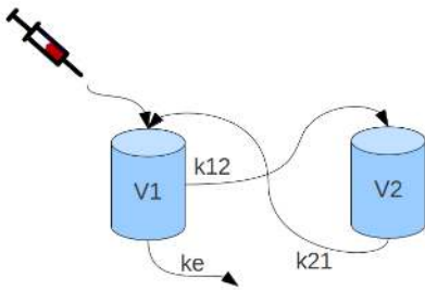
Figure 2: 2-compartment model
