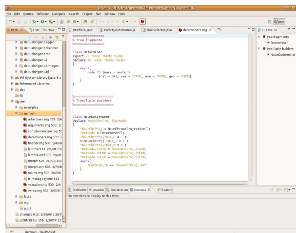
Figure 6: TuLiPA's eclipse plug-in.
