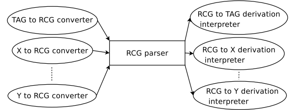
Figure 3: Towards a multi-formalism parsing environment.
