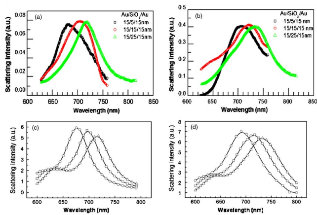
FIG. 2. (Color online) Measured scattering spectra for singlet (a) and doublet nanodisks (b) with different SiO 2 layer thicknesses: 5 nm (□), 15 nm (○), and 25 nm (△), respectively. The disk center-center spacing is 250 nm for doublets. (c), (d) Simulated scattering spectra for single nanodisks of identical sizes as in the experiments. The SiO 2 layer thickness is 5 nm (○), 15 nm (□), and 25 nm (△), respectively.
