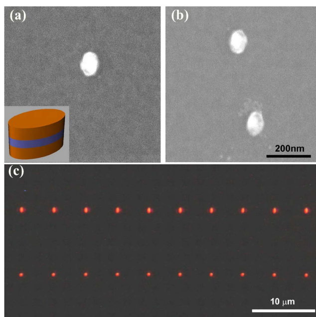
FIG. 1. (Color online) (a), (b) SEM pictures of Au/SiO 2 /Au three layered nanodisk singlet (a) and doublet (b). (c) Real color picture of nanodisks illuminated by evanescent white light waves taken with a digital camera. The top row contains doublets, and the bottom row contains singlets. The thicknesses of Au and SiO 2 disks are 15 nm and 15 nm, respectively, in all pictures here.
