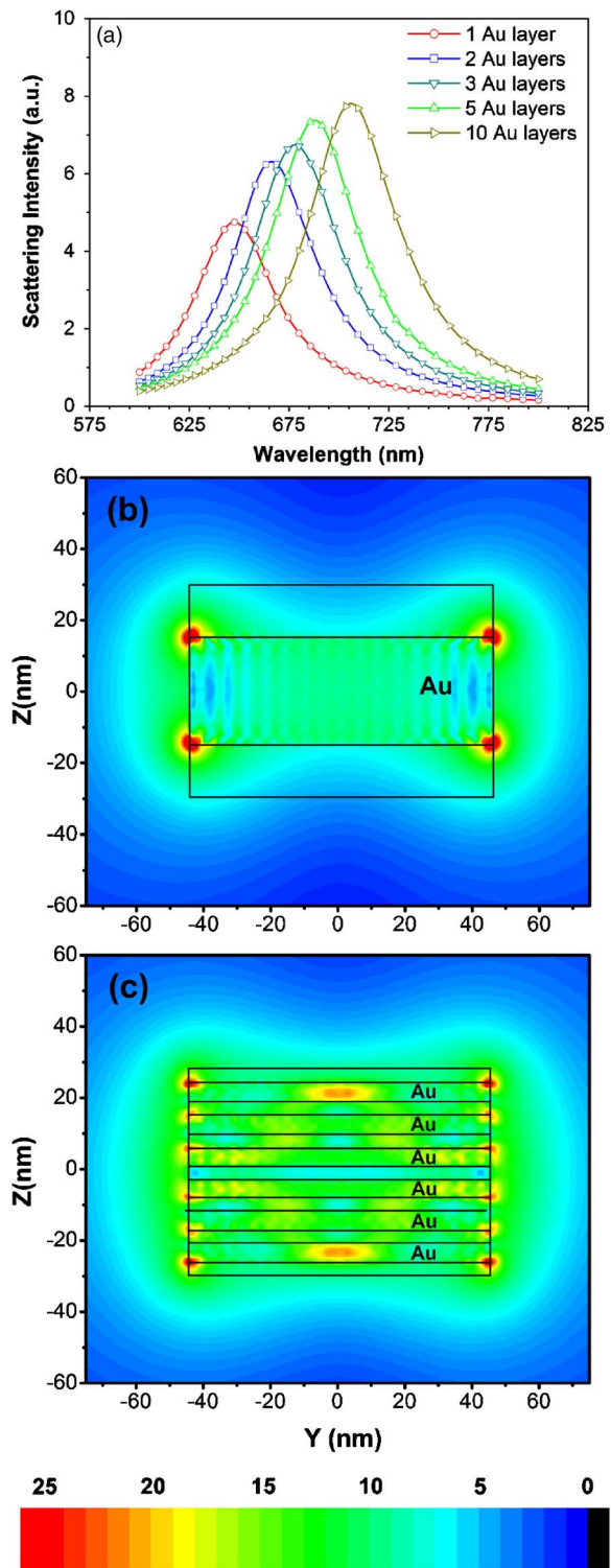
FIG. 3. (Color online) (a) Simulated scattering spectra for single nanodisks with various metal layers. The nanodisk is circular with a 90 nm diameter, while the total thicknesses for metal layers and SiO 2 layers are kept both at 30 nm. The polarization of the incident light is polarized in the Y-axis direction. (b) Y-Z plane cross section of local electrical field distribution for the single Au layer nanodisk (SiO 2 /Au/SiO 2 ) at the resonant frequency. (c) Y-Z plane cross section of local electrical field distribution for the 6 Au layer nanodisks (SiO 2 /Au) 6 /SiO 2 at resonant frequency.
