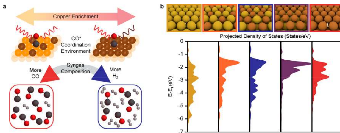
Figure 1. Cu enrichment of Au surfaces enables tuning the composition of electro synthesized syngas. (a) Scheme depicting the relationship between Cu-enriched Au surface, in situ characterization of CO* coordination, and syngas composition. (b) Calculated d-band electronic states for increasingly Cu-enriched Au surfaces.
