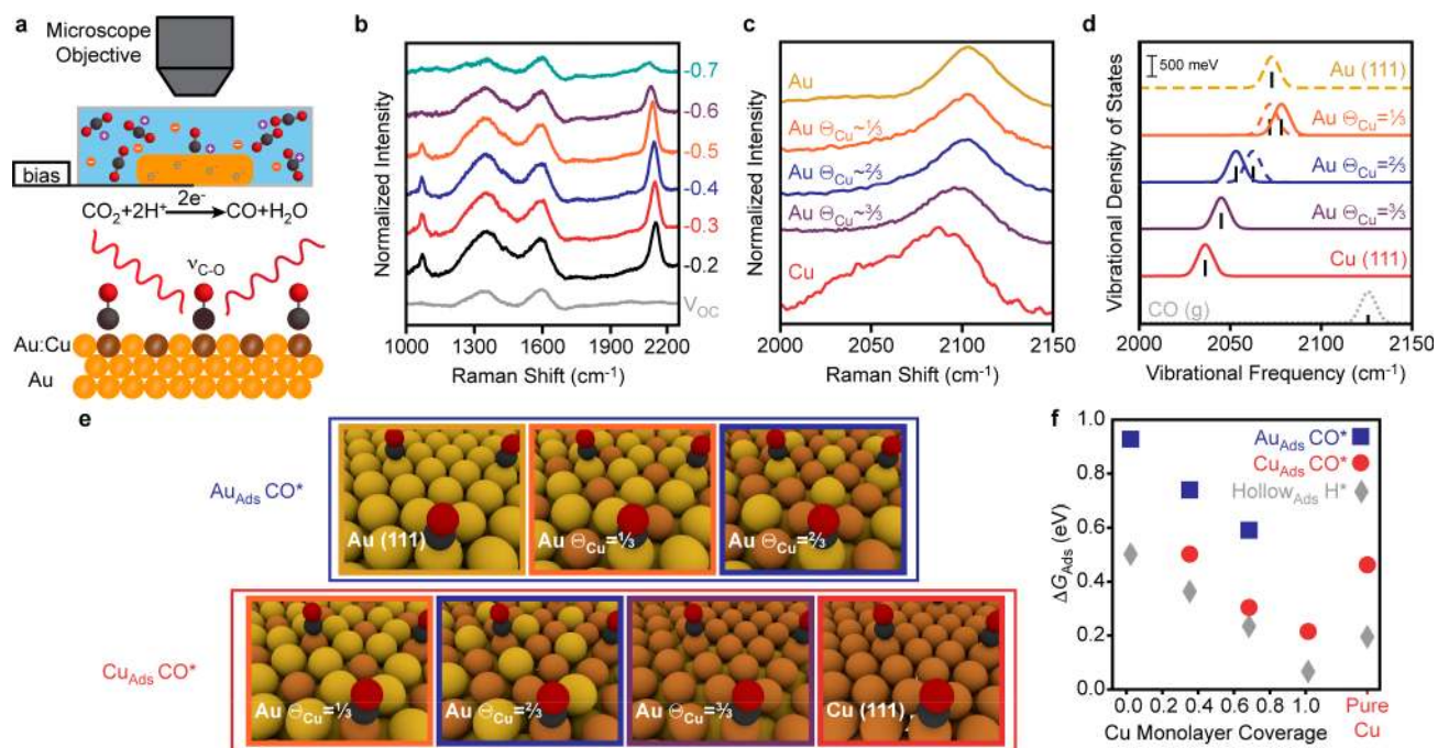
Figure 3. In situ spectroscopic and theoretical characterization of CO* binding. (a) Scheme depicting in situ SERS during CO electroynthesis. (b) Waterfall plot of typical SER spectra as a function of potential for the fully Cu enriched Au electrode (V vs RHE). (c) Waterfall plot of SER spectra for different Cu UPD coverages at -0.3 V vs RHE. (d) Calculated vibrational frequencies for CO bound on Cu-enriched Au slab models (from Figure 1). Solid lines indicate CO* at Cu sites, dashed lines indicate CO* at Au sites, and the narrow dashed trace (bottom) is for gas-phase CO at the same level of theory. (e) Renderings of optimized slab geometries for the different CO* adsorption sites. (f) Calculated adsorption energies for CO* at Au sites (blue squares) and Cu sites (red circles) as well as for H* (gray diamonds).
