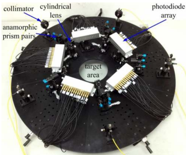
FIG. 3. Layout of the fan-beam TDLAS-based tomographic sensor.
