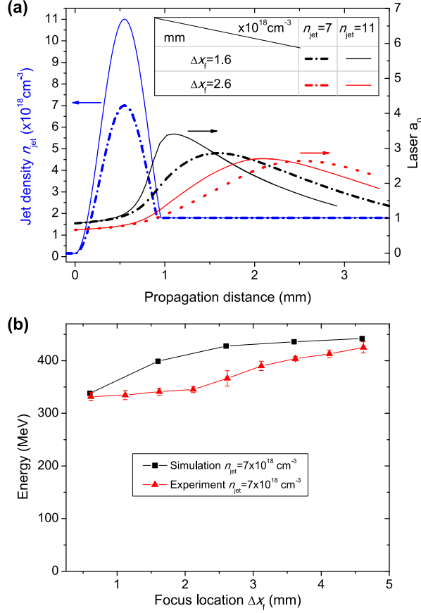
FIG. 4. Comparison of the energy gain observed in simulation and experiment, demonstrating tunability of electron beam energy via control over laser pulse diffraction. (a) Simulated evolution of the normalized vector potential a_0 as a function of propagation distance for different focal locations, \Delta x_f = 1.6 \text{ mm} (black) and \Delta x_f = 2.6 \text{ mm} (red), and peak densities, n_{\text{jet}} = 7 \times 10^{18} \text{ cm}^{-3} (dotted lines) and n_{\text{jet}} = 11 \times 10^{18} \text{ cm}^{-3} (solid lines). The blue lines shows the longitudinal density profile. (b) The energy gain computed as a function of n_{\text{jet}} for different focal locations, along with experimental data for the conditions of Fig. 2 (b-g). The error bars correspond to the standard deviation of the data.
