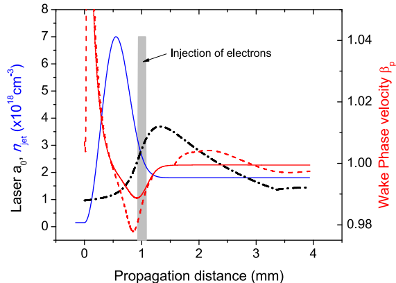
FIG. 3. Simulated evolution of the normalized vector potential a_0 (dash-dot line) as a function of propagation distance for \Delta x_f = 1.6 mm and n_{\text{jet}} = 7 \times 10^{18} cm ^{-3} . The blue solid line shows the longitudinal density profile. The phase velocity reduction (red dashed line) was larger than that for the downramp alone (red solid line) due to self-focusing increasing the non-linear plasma wavelength, and trapping of electrons occurred in the grey shaded area. The phase velocities shown are measured in the center of the bubble behind the laser pulse where the longitudinal electric field is 0. The phase velocity reduction at the back of the bubble is approximately a factor of 2 larger.
