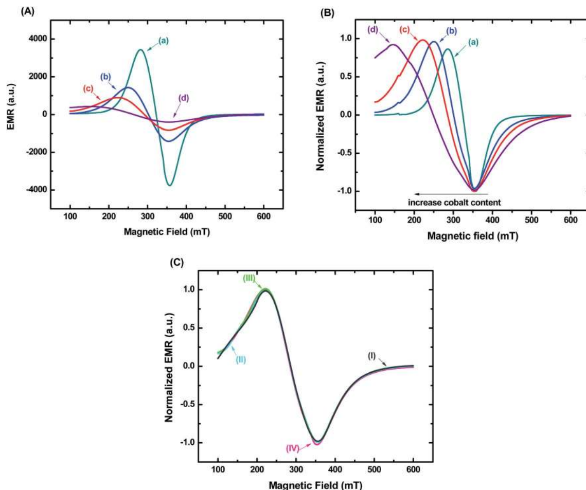
Fig. 7 EPR spectra of (a) MION@CMC, (b) Co 3 -MION@CMC, (c) Co 5 -MION@CMC, and (d) Co 10 -MION@CMC for (A) samples in powder form and (B) ferrofluids. (C) EPR spectra of Co 5 -MION@CMC ferrofluids with (I) 0.1 mg mL -1 , (II) 0.5 mg mL -1 , (III) 1.0 mg mL -1 and (IV) 5.0 mg mL -1 .
