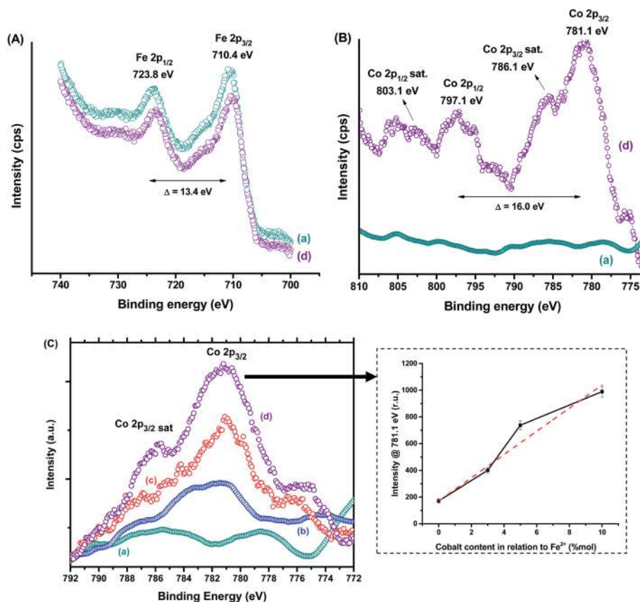
Fig. 3 XPS spectra of (A) Fe 2p and (B) Co 2p regions for (a) MION@CMC and (d) \text{Co}_{10} -MION@CMC. (C) Spectra of Co 2p 3/2 region for (a) MION@CMC, (b) \text{Co}_3 -MION@CMC, (c) \text{Co}_5 -MION@CMC, and (d) \text{Co}_{10} -MION@CMC. Inset: evolution of intensity at Co 2p 3/2 peak with increasing cobalt content.
