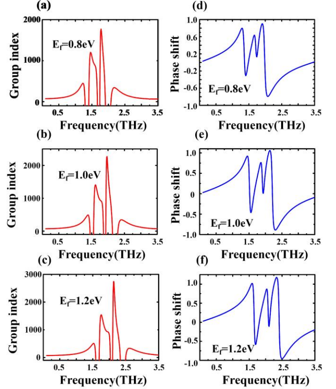
Figure 7. (a-c) Group index of the proposed metamaterials at different Fermi Levels; (d-f) Phase shifts of the proposed metamaterials at different Fermi levels.
