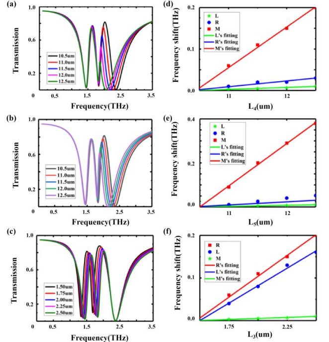
Fig. 4 Evolution of the PIT curve when the longitudinal length L_4 (a) and the longitudinal length L_5 (b) of the lower layer of square ring graphene and the crosswave length L_3 (c) of upper graphene band; (d-f) Frequency shifts of three resonant frequencies versus changes the geometric parameters of the graphene structure.
