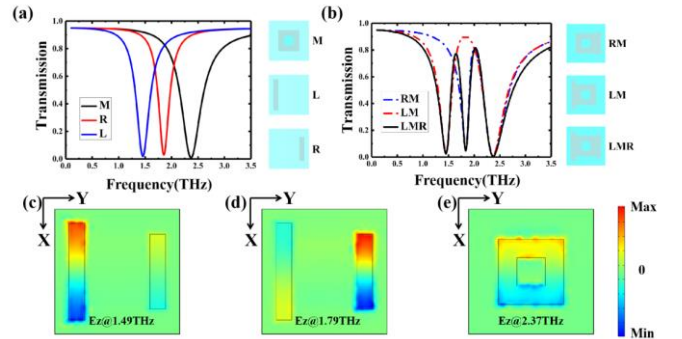
Fig. 2 (a) Simulated transmission spectra of single M, Single L and single R metamaterials; (b) Simulated transmission spectra of proposed metamaterial LMR, Single LM, and single RM metamaterial structures. Here, Fermi levels of graphene are both 1.2 eV; (c) Ez distribution of three resonant frequencies in the transmission spectrum of the material.
