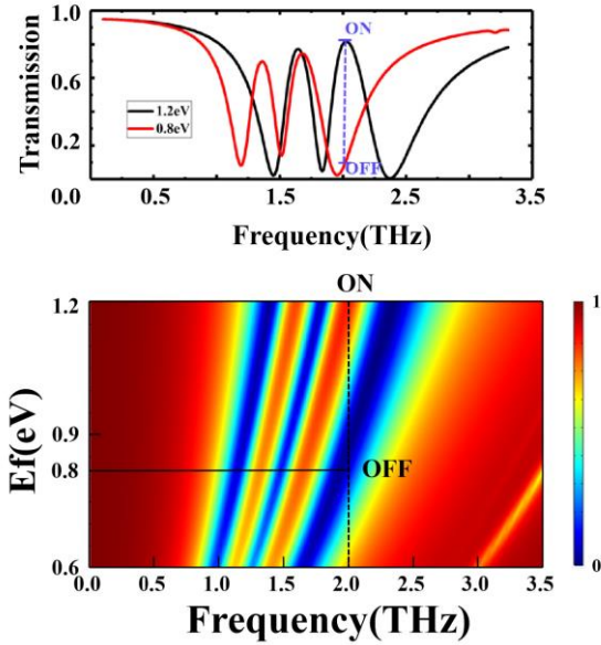
Figure 6. (a) Modulation mechanism of electro-optical switch; (b) Three dimensional modulation diagram at different graphene Fermi levels.
