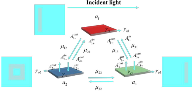
Fig. 3 Coupling model of three resonance modes.
