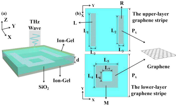
Fig. 1 (a) Schematic diagram of graphene metamaterial on SiO 2 substrate; (b) Top view of metamaterial's structural unit; and size: L_1=15.5 \mu\text{m} , L_2=12 \mu\text{m} , L_3=2.5 \mu\text{m} , L_4=L_5=10.5 \mu\text{m} , L_6=L_7=4.5 \mu\text{m} , d=1.2 \mu\text{m} , P_x=20 \mu\text{m} .
