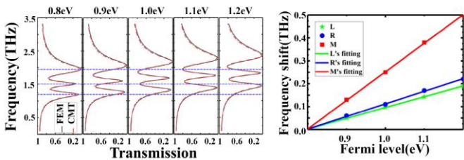
Fig.5 (a) The PIT transmission spectra of numerical simulation and fitting at the different Fermi levels of graphene. (b) Frequency shifts of three resonant frequencies versus Fermi level.
