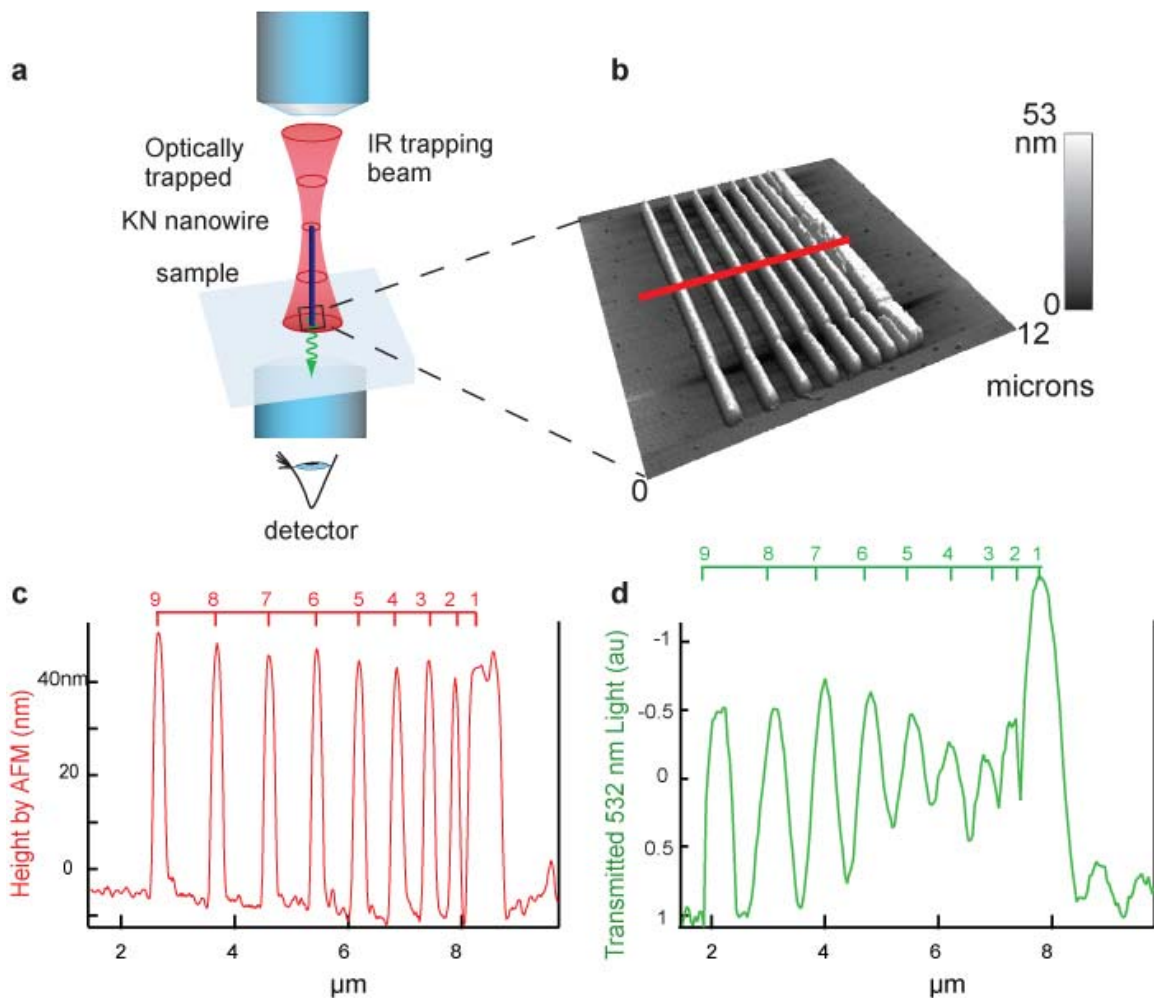
Figure 3 | Transmission line scan of metallic surface pattern with laser trapped \text{KNbO}_3 nanowire. a , Schematic of inverted optical scanning configuration. b , AFM topographic image of thermally evaporated pattern of gold stripes on a glass coverslip. c , AFM line scan from region indicated in (b) d , Optical transmission profile captured by scanning a single \text{KNbO}_3 nanowire over the metallic surface structure. The nanowire used to create the transmission line scan was measured by AFM to have the dimensions: width=122 nm, length =1.4 \mu\text{m} and height=53 nm.
