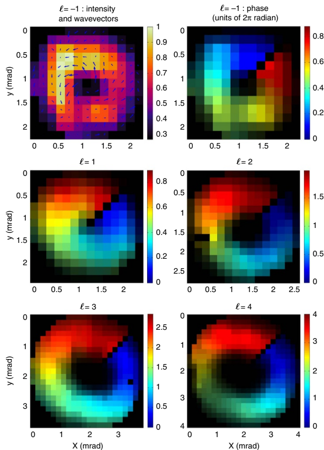
Figure 3 | Intensity and wavefront measurements for several modes carrying various topological charges. The top-left panel shows the intensity (in arbitrary units) and the local wavevector (arrows) distribution for the \ell = -1 mode of the 16th high-harmonic order emission (h16). The other panels show the measured wavefronts for \ell = -1 and \ell = 1 for h16, \ell = 2 for h19, \ell = 3 for h18 and \ell = 4 for h19 (intensity and wavevector distribution for the latter cases is shown in Supplementary Fig. 1). The intensity is represented by the brightness (in units of 2\pi radian) by false colours. Black colour indicates pixels that contain no data (intensity lower than the detection threshold or pixels set to zero to enable wavefront reconstruction around the singularity). Note that the different panels have different colour scales. The yield of each individual mode was optimized (see next section), and a crossing angle of 15 mrad was used to guarantee a larger spatial separation between the modes, compared to the one in Fig. 2.
