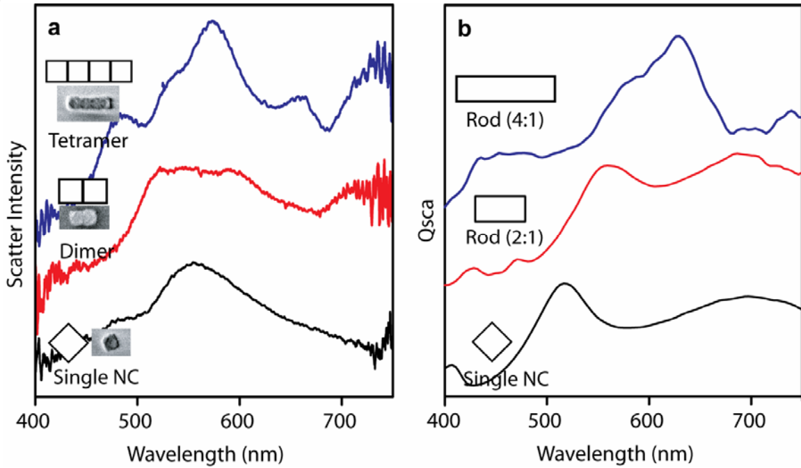
Fig. 4. Optical response of Ag NC oligomers. (a) Darkfield scattering spectra of NC oligomers collected in transmission mode after dispersing a droplet of the colloidal solution onto a glass slide patterned with alignment marks. The number of identifiable plasmon modes increases as oligomer size increases, indicating strong electromagnetic coupling between neighboring cuboctahedra. SEM images show that within the groups, the NCs are in intimate contact with each other (spacing < 5 nm). (b) Discrete dipole approximation simulations corresponding to the NC oligomers studied in (A). Cuboctahedra dimers and tetramers are modeled as corrugated rods with aspect ratios of 2:1 and 4:1, respectively.
