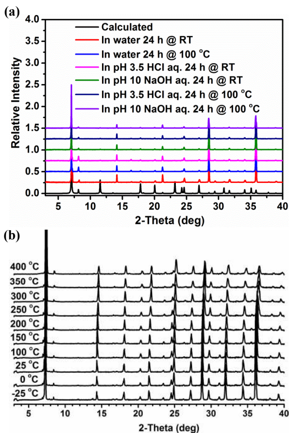
Figure 2. PXRD patterns for 1 : after treatment in water, acidic and basic conditions for 24 h at room temperature and 100 °C, respectively (a), and in-situ variable temperature (VT) under a vacuum (b).
