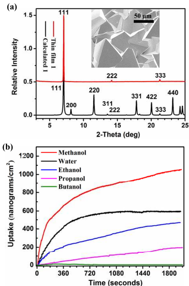
Figure 6. PXRD patterns of 1 calculated and thin-film grown on the -OH -terminated self-assembled monolayer surface (inset is SEM image of thin-film 1 after 24 h of growth) (a) and QCM profiles of specific mass uptake of VOCs at the saturated vapor pressure at room temperature for thin film 1 (b).
