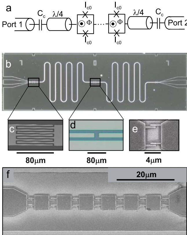
Fig. 1 (a) Tunable resonator scheme: a DC SQUID array is inserted between two \lambda/4 waveguides coupled to a 50 \Omega measurement line through input and output capacitors C_c . (b) Optical micrograph of a CPW niobium resonator. (c) Typical coupling capacitor (design value: C_c = 27 fF). (d) Gap in the middle of the resonator, before SQUID patterning and deposition. (e) Electron micrograph of an aluminum SQUID (sample A), fabricated using electron-beam lithography and double-angle evaporation. (f) Electron micrograph of a 7-SQUID array (sample B)
