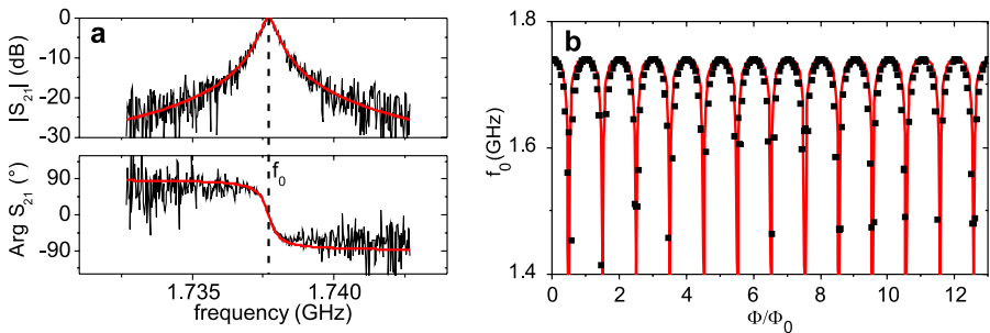
Fig. 4 (Color online) (a) Measured (thin line) amplitude (top) and phase (bottom) transmission of sample A for \Phi = 0 and fit (bold line) yielding the resonance frequency f_0 and a quality factor Q = 3300 . (b) Measured f_0 of sample A (squares) as a function of applied magnetic flux, and corresponding fit (full line) according to (7)
