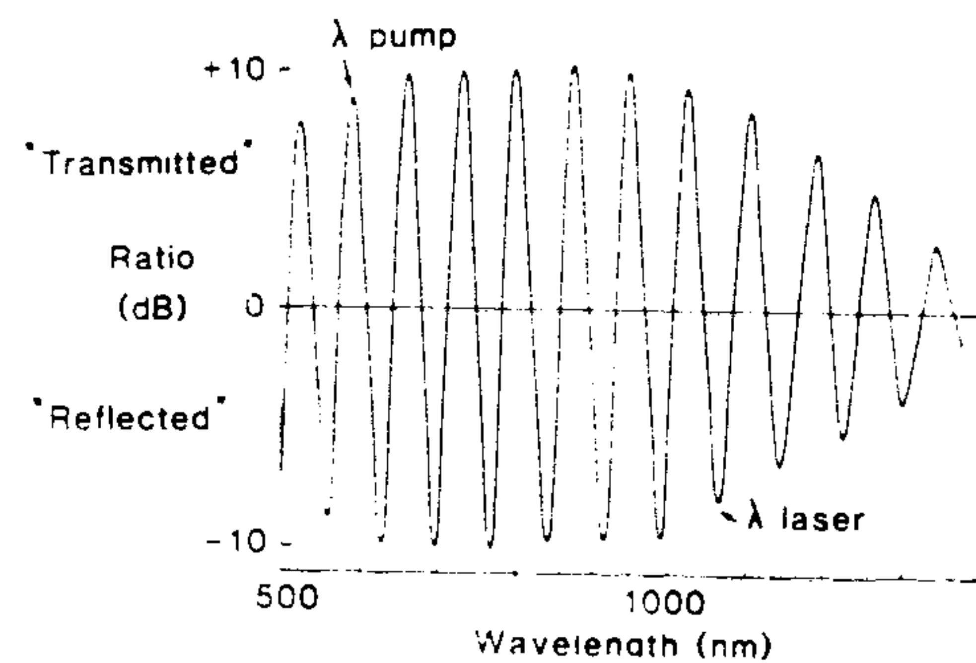
Fig. 3. Wavelength coupling characteristic of ring resonator fiber coupler.
