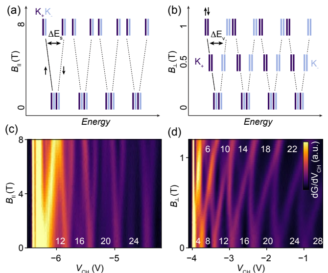
FIG. 2. (a)(b) Schematic for the lifting of degeneracies in parallel/perpendicular B of the subbands in the QPC. For B_{\parallel} the valleys do not split. In B_{\perp} the valley splitting exceeds the spin splitting by far. (c) dG/dV_{CH}(V_{CH}, B_{\parallel}) of QPC2 at (V_{BG}, V_{SG}) = (7, -4)V . (d) dG/dV_{CH}(V_{CH}, B_{\perp}) of QPC3 at (V_{BG}, V_{SG}) = (4.5, -2.93)V . The number indicates the quantized conductance in units of e^2/h .
