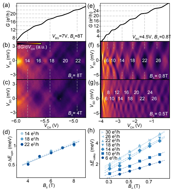
FIG. 3. (a)(e) G(V_{CH}) at B_{\parallel} = 8\text{ T} and (V_{BG}, V_{SG}) = (7\text{ V}, -4\text{ V}) in QPC2 and at B_{\perp} = 0.8\text{ T} and (V_{BG}, V_{SG}) = (4.5\text{ V}, -2.93\text{ V}) in QPC3. (b)(c) dG/dV_{CH}(V_{CH}, V_{sd}) at B_{\parallel} = 8\text{ T} and 4\text{ T} , respectively. The plot shows spin-split energy levels. Diamonds at 14, 18, 22 e^2/h grow larger in size with increasing B . (f)(g) dG/dV_{CH}(V_{CH}, V_{sd}) at B_{\perp} = 0.8\text{ T} and 0.5\text{ T} , respectively. (d) Energy spacings \Delta E_{\text{spin}} , extracted from the height of the diamonds at 14, 18, 22 e^2/h show a linear dependence on B_{\parallel} . In a similar fashion the energy spacings \Delta E_{\text{valley}}(B_{\perp}) are extracted from plots as the ones shown in (f) and (g). Dashed lines are linear fits.
