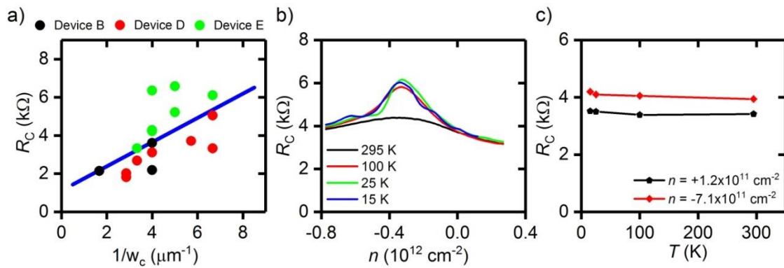
Figure S4. 1D magnetic contacts. a , Contact resistance scaling with the inverse of the contact width. R_C is taken at 20 K and at moderate carrier density n - n_0 \approx +1.5 \times 10^{12} \text{ cm}^{-2} , where n_0 is the carrier density at the R_C maxima. The blue line is a global linear fit of the data. b , Contact resistance as a function of carrier density, for different temperatures. c , Contact resistance as a function of temperature at two fixed carrier densities, for the same data as in b .
