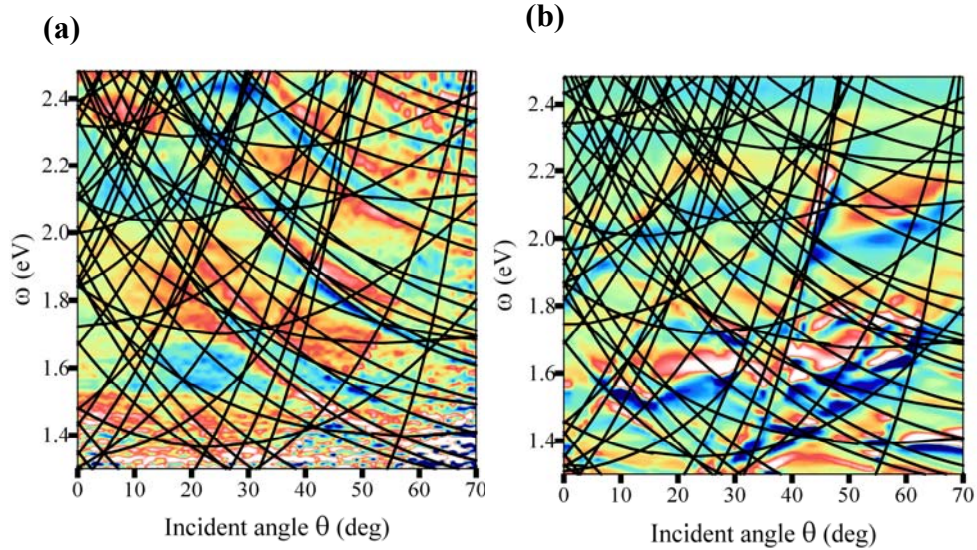
Fig. 4. Experimental angular dispersion for (a) uncoated and (b) Au-coated pit arrays, together with theoretical diffraction modes. The dynamic range in (a) is 10 times less than in (b). Animated data of (a) as a function of azimuthal angle is available as a multimedia file (2.5Mb)
