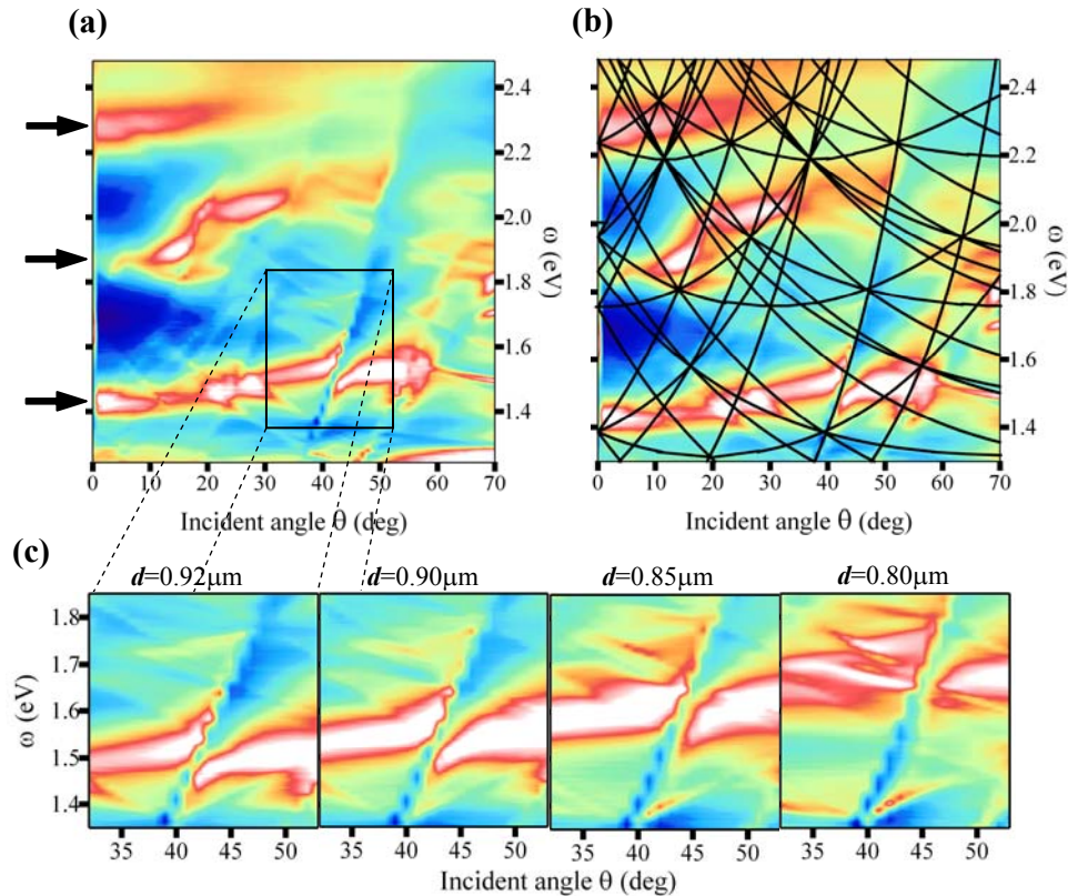
Fig. 6. (a) Angular dispersion of reflectivity on Au-coated pit array for \phi=45^\circ and d=920\text{nm} , with (b) superimposed diffraction curves. (c) Strong coupling observed in angular dispersion of samples with increasing pit depth. Animation of (b) as a function of decreasing pit depth is available as a multimedia file (1Mb)
