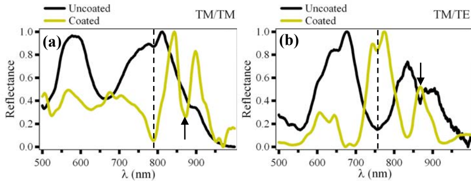
Fig. 2. Reflection spectra at 50^\circ incidence and 3^\circ azimuthal angle for a square array of silicon pits which are uncoated (black) and gold-coated (yellow). (a) TM incident, TM analysed, (b) TM incident, TE analysed. Dotted lines are diffraction features, arrows mark plasmons.
