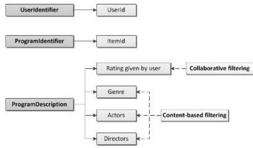
Figure 2 Metadata schema
