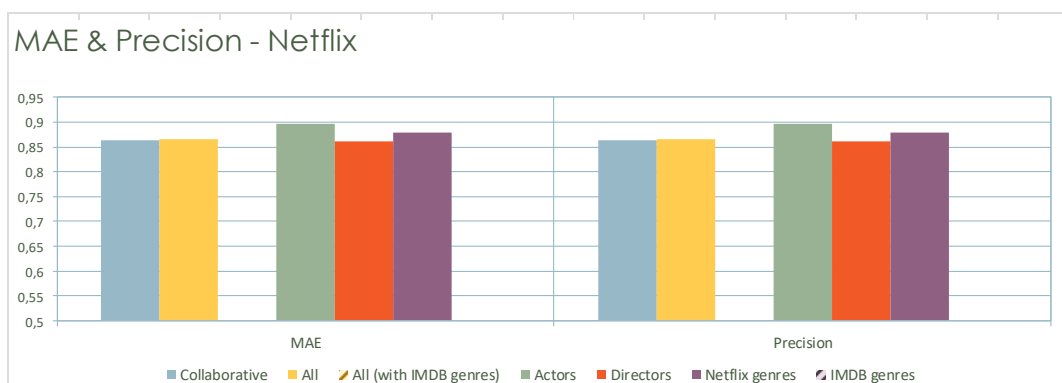
Figure 10 - MAE and Precision comparing algorithm’s performance using original Netflix genres against IMDB genres (chronological partition).
