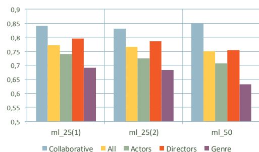
Figure 4 - MAE and Precision for the MovieLens dataset (partition based on the number of ratings)
