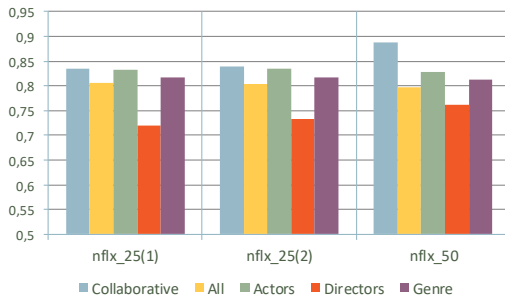
Figure 3 - MAE and Precision for the Netflix dataset (partition based on the number of ratings)
