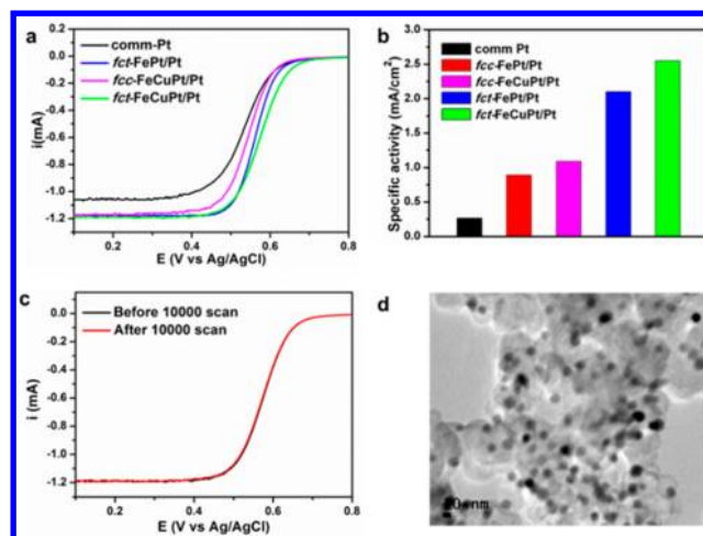
Figure 6. (a) ORR polarization curves of Pt, fct-FePt/Pt, fcc-FeCuPt/Pt, and fct-FeCuPt/Pt NPs. (b) The specific activities of the NP catalysts at 0.531 V ( E_{1/2} of the commercial Pt catalyst). (c) ORR polarization curves of the fct-FeCuPt/Pt NPs before and after 10 000 potential scans between 0.4 and 0.7 V. (d) TEM image of the fct-FeCuPt/Pt NPs after 10 000 potential scans.
