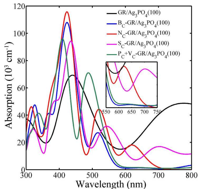
Figure 7. Absorption spectra of the undoped, B_C -, N_C -, S_C -, and P_C+V_C -GR/Ag 3 PO 4 (100) composites for the polarization vector perpendicular to the surface. The inset shows that the N_C - and S_C -GR/Ag 3 PO 4 (100) composites display strong absorption in the range 550 to 750 nm. The higher resonant-like peaks at about 400–440 nm, due to doping, are especially beneficial to enhance the photocatalytic performance of the doped GR/Ag 3 PO 4 (100) composites, according to the fact that the light with wavelength of ~440 nm might be the most appropriate visible light for generation of radical species in the GR/Ag 3 PO 4 (100) composite. The N atom may be one of the most appropriate dopants for the GR/Ag 3 PO 4 photocatalyst.
