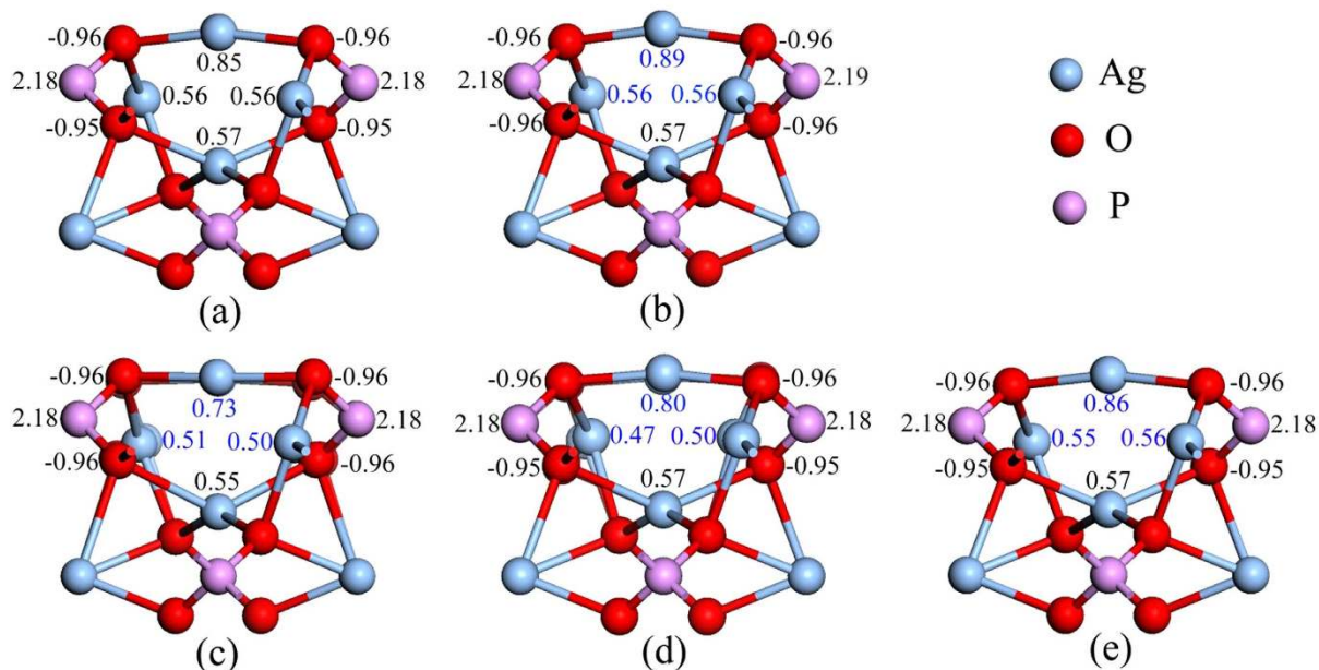
Figure 4. The Mulliken population charges on Ag, O, and P atoms, which have changed in the \text{Ag}_3\text{PO}_4(100) surface. (a–e) are for undoped, \text{B}_\text{C} -, \text{N}_\text{C} -, \text{S}_\text{C} -, and \text{P}_\text{C} + \text{V}_\text{C} -doped \text{GR}/\text{Ag}_3\text{PO}_4(100) composites, respectively. The blue digits represent the changed Mulliken population charges on Ag atoms near the interface. The variation of Mulliken population charges on P atoms shows that the dopants in GR sheets change the charge redistribution of the \text{Ag}_3\text{PO}_4(100) surface.
