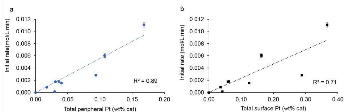
Figure 6. The correlation between the 3-NS initial conversion rate and total amount of Pt present in (a) peripheral sites and (b) as exposed surface atoms for the different Pt/TiO 2 catalysts as estimated from analysis of HAADF-STEM images. For model (a) R^2 = 0.89 , p < 0.001 , and for model (b) R^2 = 0.71 , p < 0.02 .
